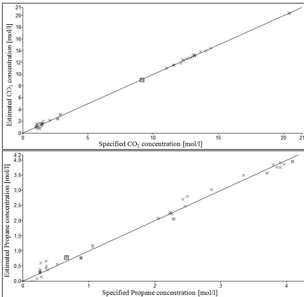
Figure 9: Estimated versus specified concentrations of CO 2 and propane
