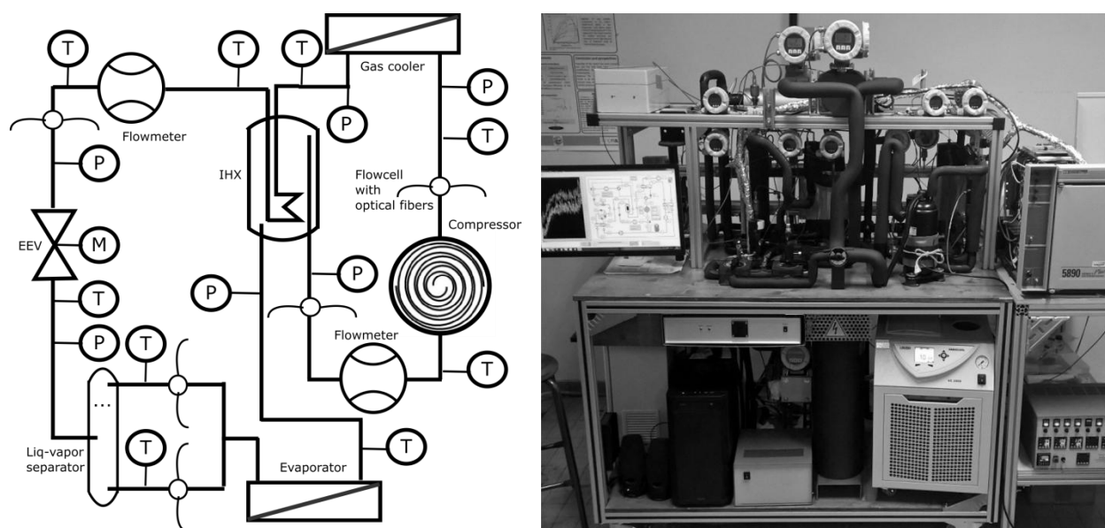
Figure 3: Heat pump loop and experimental bench
