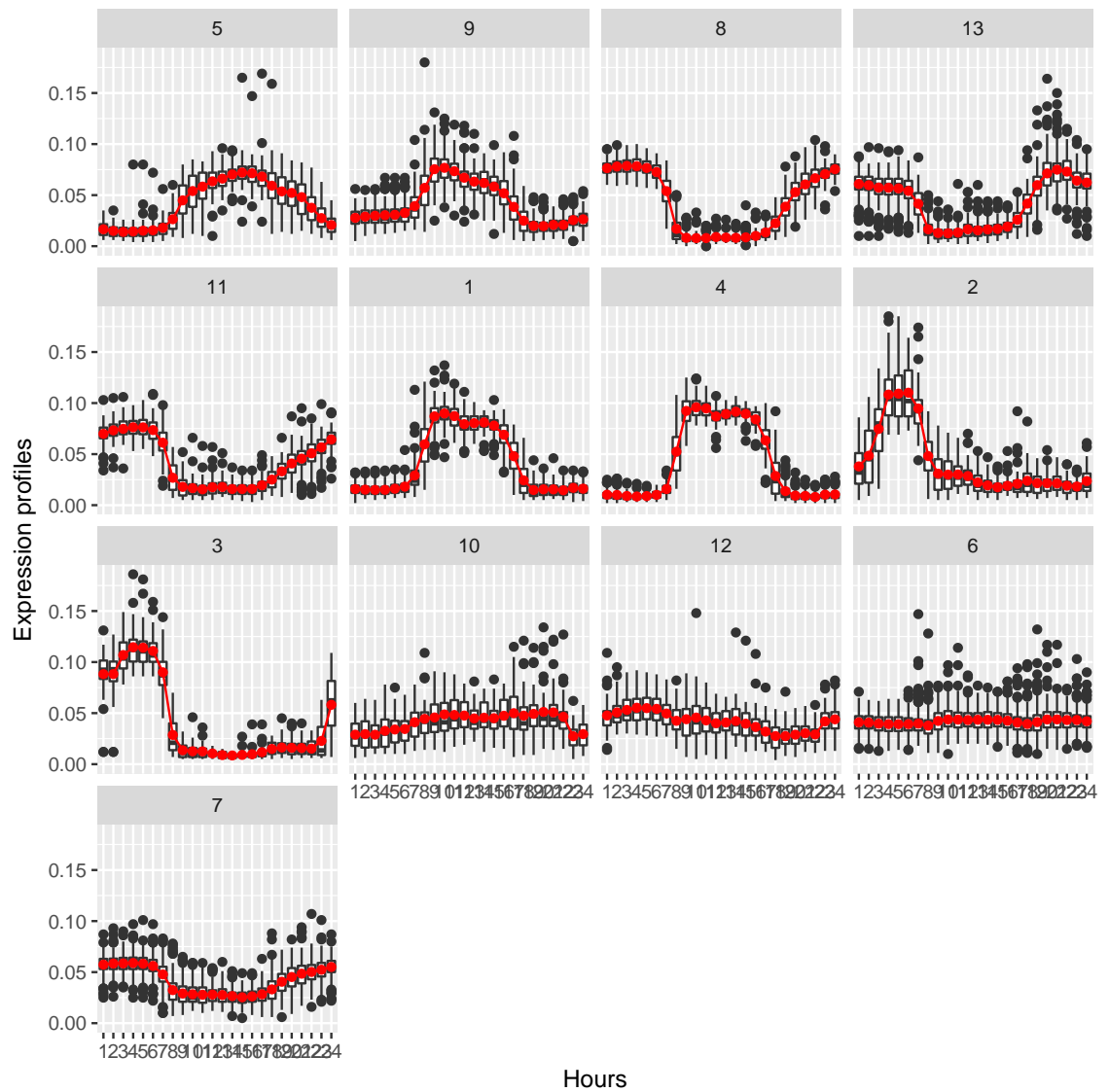
FIG 22. Clusters of genes from the Velib' bicycle sharing system data: per-cluster occupancy profiles of selected clusters obtained with the K-means algorithm and logCLR transformation. Clusters have been arranged so that those with similar average profiles are displayed next to one another. Connected red lines correspond to the mean profiles for each time point.
