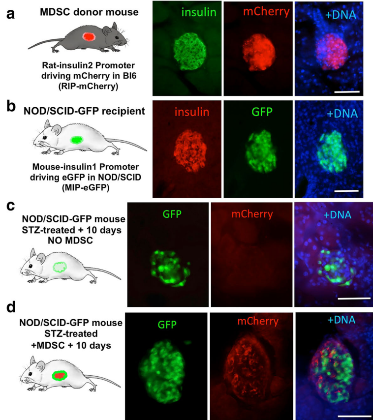
Fig. 6 Muscle-derived stem cells (MDSC) differentiate in vivo into insulin-expressing cells 10 days after intraperitoneal injection in streptozotocin (STZ)-treated mice. To examine if undifferentiated MDSC could differentiate in vivo into functional beta cells, MDSC were isolated from a donor mouse expressing mCherry under the control of the rat INS2 promoter that expressed mCherry specifically in pancreatic beta cells as shown by co-immunostaining for insulin (green) (a). Recipient NOD-SCID-MIP-eGFP transgenic mice expressed eGFP under the control of the mouse INS1 promoter specifically in pancreatic beta cells as shown by co-staining for insulin (red) (b). Recipient MIP-eGFP mice were injected with the glucose analog STZ to destroy endogenous beta cells and 60 min later with either saline vehicle (STZ only) or MDSC (STZ + MDSC), and pancreatic vibratome sections were analyzed 10 days later. Panels in (c) show staining for eGFP (green) and mCherry (red, no signal) in a pancreatic islet of MIP-eGFP mouse 10 days after STZ injection alone. Panels in (d) show staining for eGFP (green) and mCherry (red) in an islet of MIP-eGFP mouse 10 days after injection of STZ and undifferentiated muscle stem cells from a RIP-mCherry donor mouse. Scale bars = 100 \mu m
