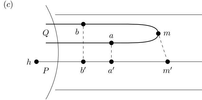
■ Figure 6 Proof of Lemma 21
