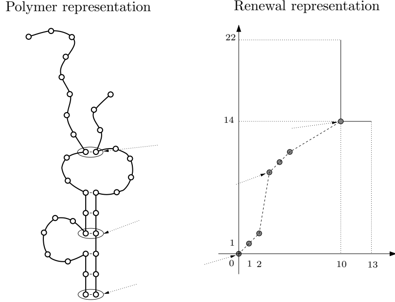
FIGURE 1. A configuration of the gPS model, with one strand containing 23 bases and the other 14, is represented in two fashions: the natural (or polymer) one and the renewal one. In particular we see that (1, 1) renewal increments (or inter-arrivals) correspond to bound base pairs and all other increments (i, j) correspond to unbound regions in the bulk, that we call loops (of total length i + j , with length i in the first strand and j in the second strand). The term unbound is rather reserved to the terminal portion of the polymer: we refer the free ends as unbound strands. Throughout this work, a polymer trajectory is always given in the renewal representation: it is therefore just a point process in the plane.
