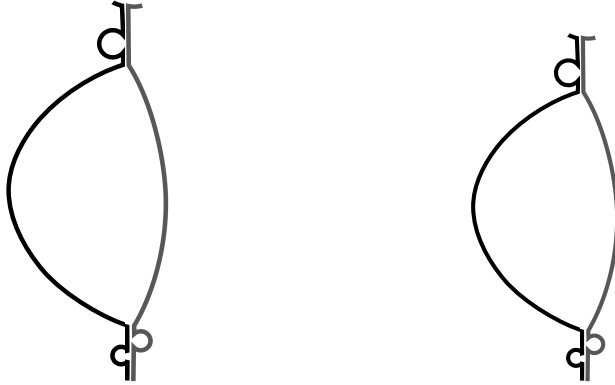
FIGURE 2. A schematic image of the two types of observable trajectories of the free gPS model in the delocalized (denaturated, melted) regime, according to whether the exponent \bar{\alpha} is smaller (left picture) or larger (right picture) than 1 + \alpha/2 . In the constrained case only the trajectory on the right is observed, and the small free tails are reduced to zero. This case is treated in [12].
