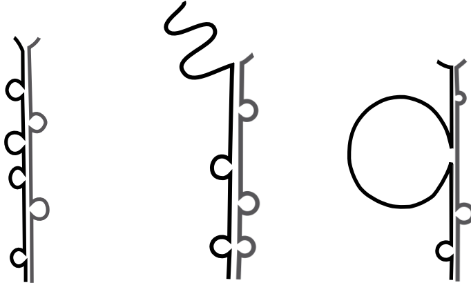
FIGURE 3. Schematic image of the observable trajectories of the free gPS model in the Cramér regime (left), and in the non-Cramér regime (cf. Theorem 1.1): the Large Unbound Strand event (center, occurring when \bar{\alpha} < \alpha + 1 ) and the Big Loop event (right, occurring when \bar{\alpha} > \alpha + 1 ). In the constrained case the Unbound Strand event is not observed, and the free tails are of course absent. What cannot be appreciated in this schematic view is the fact that the small loop distribution has exponential tail in the Cramér regime (hence the largest is O(\log N) ) and that it has power law tail in the non-Cramér regime (hence the largest is O(N^a) for some a \in (0, 1) : O(m_N) to be precise).
