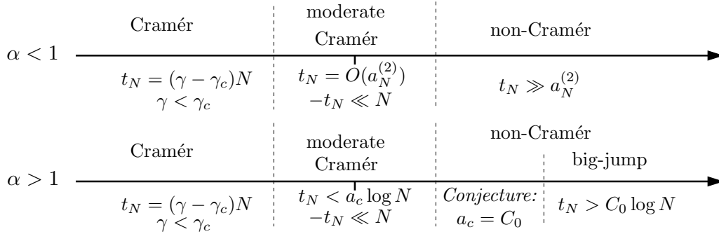
FIGURE 4. A schematic sum-up of the correspondence of the values of t_N = (\gamma - \gamma_c)N with the different regimes. We treat the big-jump domain and it is the one to the right of the right-most dashed line. We believe that to the right of the moderate Cramér regime there is the big-jump domain — put otherwise, the non-Cramér regime coincides with the big-jump domain — but this is proven only for \alpha < 1 .
