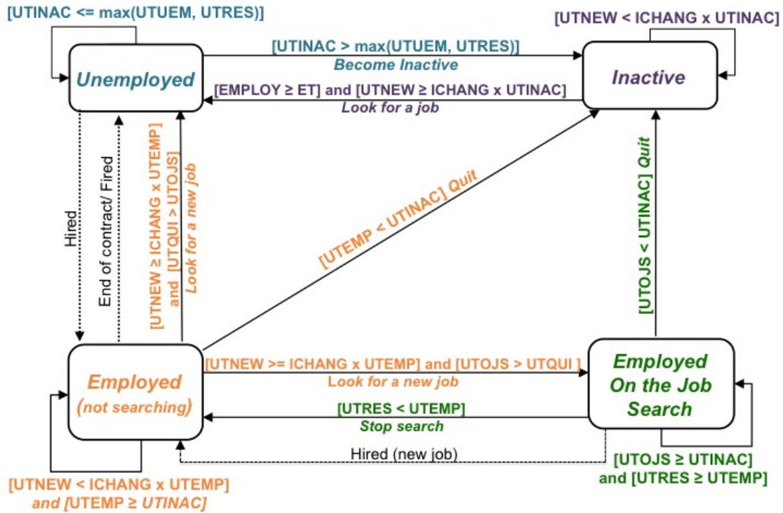
Fig. 3: UML State diagram describing the main transitions of individuals and their decision-making process. UTTINA: utility to be inactive. UTNEW: utility of a new job, estimated through prospecting. UTUEM: utility to be unemployed. UTRES: utility of reservation. UTOJS: utility of the OJS (On-the-Job-Search) state. UTEMP: utility to be employed. UTQUI: utility to quit. ICHANG psychological cost to change state (calibrated exogenous parameter). EMPLOY measures the employability of the inactive. Dotted arrows represent decisions that do not fully depend on the agent (i.e. taken by the firm.)
