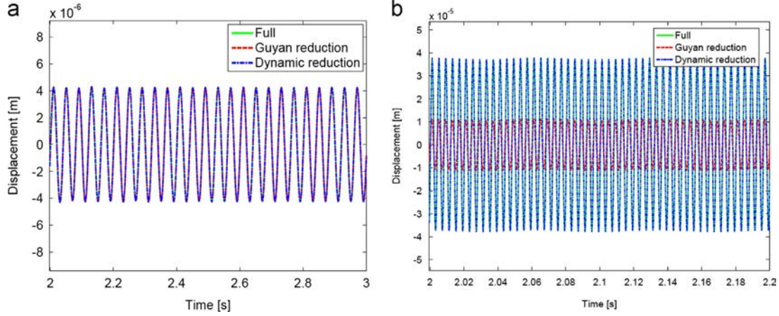
Fig. 10. Steady state responses for full and reduced models: dynamic/Guyan reduction methods of viscoelastic sandwich beam: (a) ( f < f_c ) and (b) ( f > f_c ).
