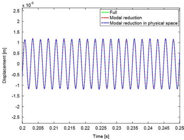
Fig. 18. Steady state response for the full and reduced models: Modal/Modal in physical space methods of the viscoelastic sandwich plate.
