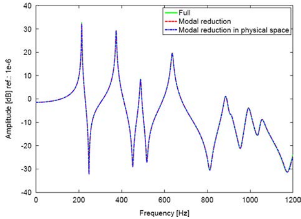
Fig. 16. FRFs for full and reduced models: Modal/Modal reduction in physical space methods for the viscoelastic sandwich plate.
