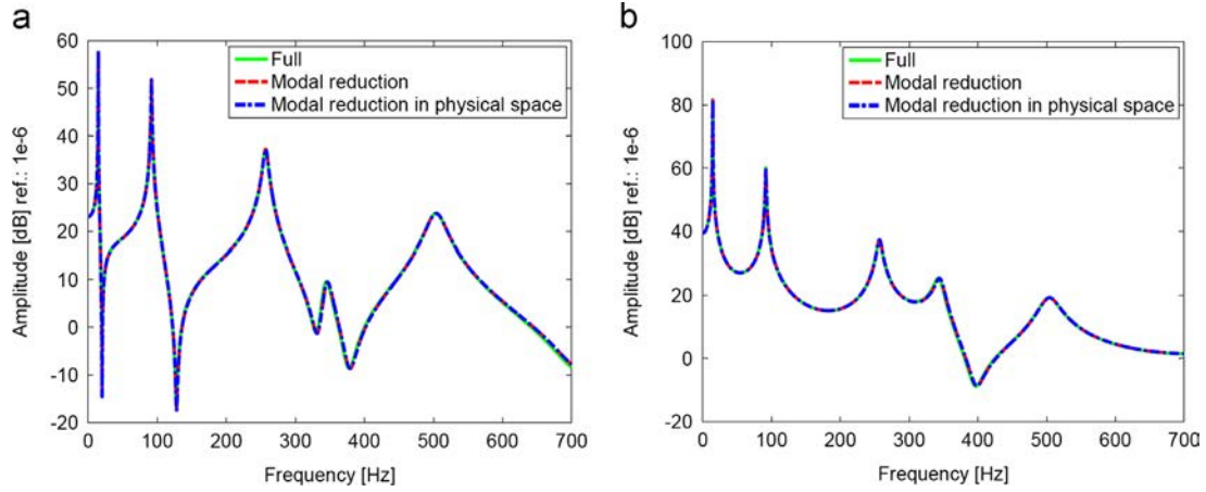
Fig. 8. FRFs for full and reduced models: Modal/Modal in physical space reduction methods: (a) point P and (b) point K of the viscoelastic sandwich beam.
