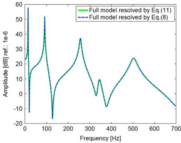
Fig. 5. FRFs of full model derived from two mathematical tools.
