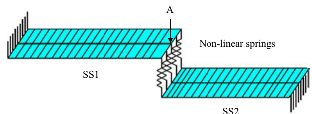
Fig. 19. FE model of the global non-linear assembled viscoelastic sandwich beam.
