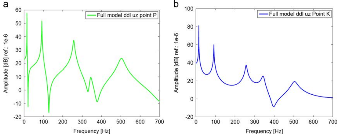
Fig. 4. FRFs of the full GHM model plotted in (a) point P and (b) point K.
