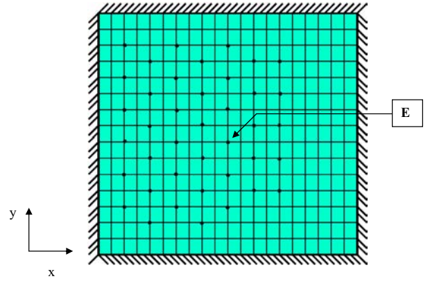
Fig. 14. FE model for the viscoelastic sandwich plate with the position of the optimal master dofs (•).
