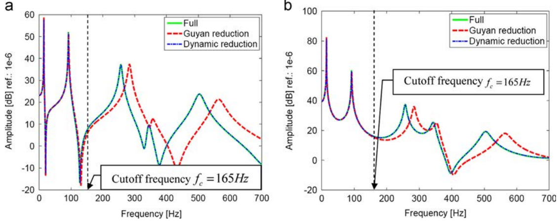
Fig. 7. FRFs for full and reduced models: dynamic/Guyan reduction methods: (a) point P and (b) point K of the viscoelastic sandwich beam.
