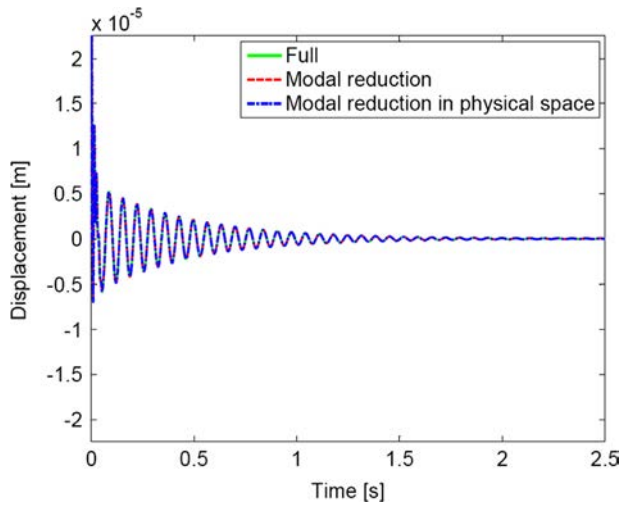
Fig. 13. Transient responses for full and reduced models: Modal/Modal in physical space reduction methods of the viscoelastic beam.
