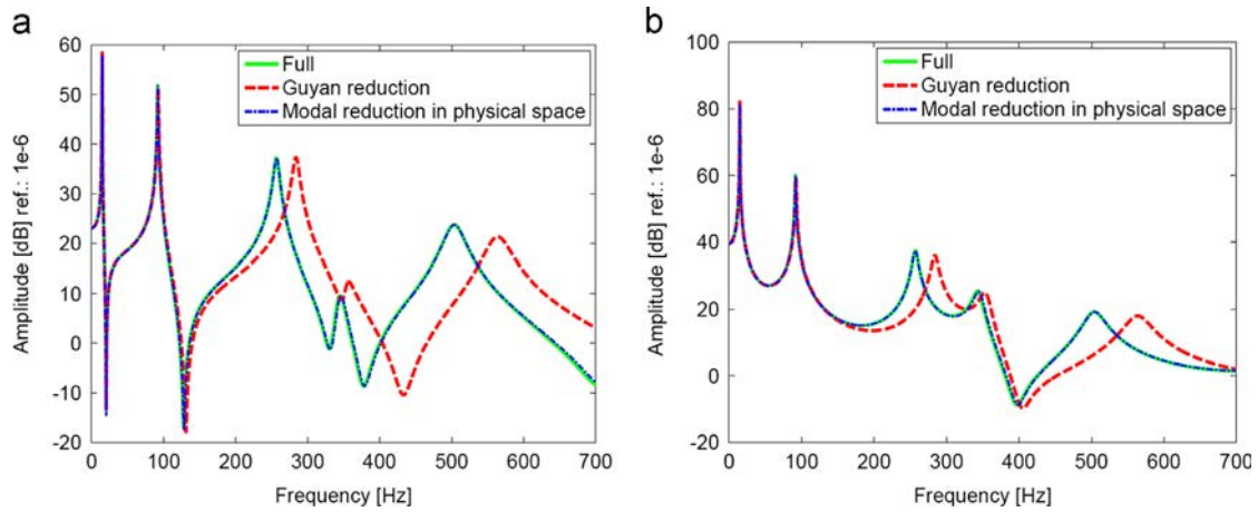
Fig. 9. FRFs for full and reduced models: Guyan/Modal in physical space reduction methods: (a) point P and (b) point K of the viscoelastic sandwich beam.
