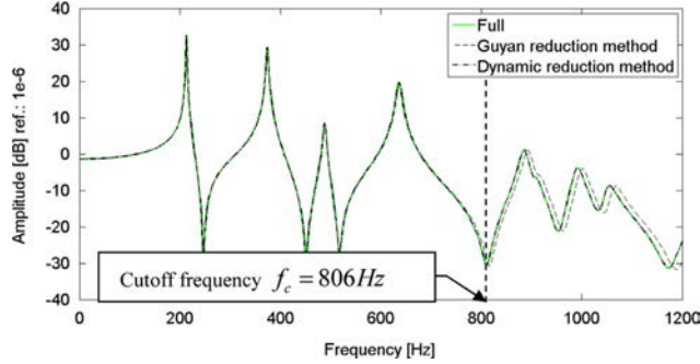
Fig. 15. FRFs for full and reduced models: Guyan/dynamic reduction methods for the viscoelastic sandwich plate.
