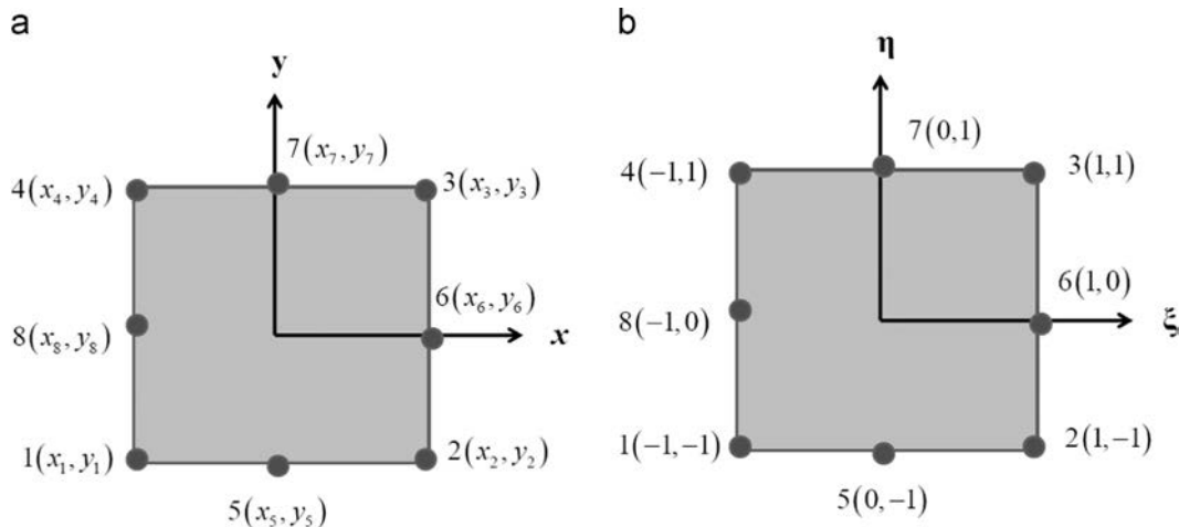
Fig. 2. Serendip finite element in (a) elementary coordinates and (b) local coordinates.
