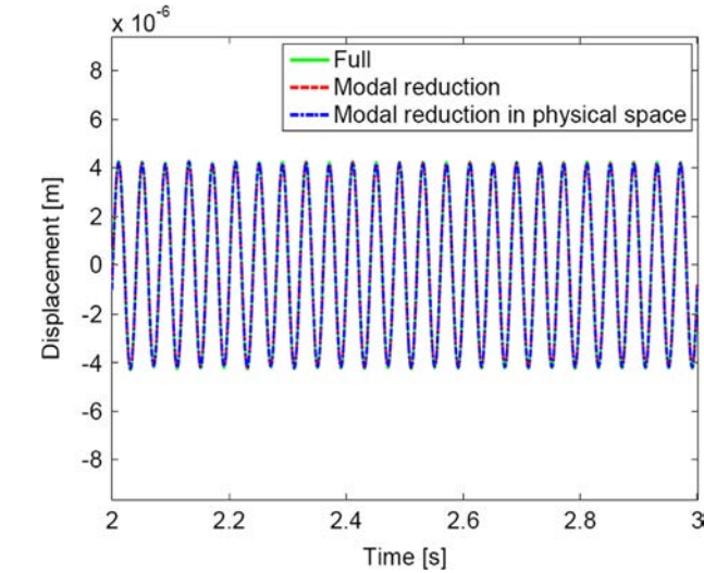
Fig. 11. Steady state responses for full and reduced models: Modal/Modal in physical space reduction methods of the viscoelastic sandwich beam.
