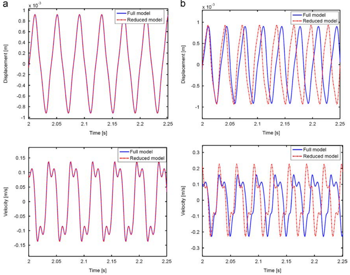
Fig. 20. Temporal responses of full and reduced models of the non-linear assembled viscoelastic sandwich beam: (a) f < f_c and (b) f > f_c .
