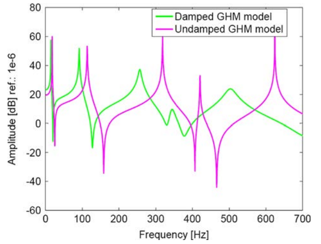
Fig. 6. FRFs of the damped and the undamped GHM model for the sandwich beam.
