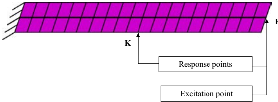
Fig. 3. Clamped-free (C-F) sandwich beam finite element.
