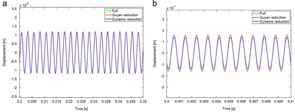
Fig. 17. Steady state response for the full and reduced models: Guyan/dynamic methods of the viscoelastic sandwich plate: (a) f < f_c and (b) f > f_c .
