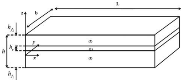
Fig. 1. Sandwich structure geometry.
