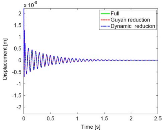
Fig. 12. Transient responses for full and reduced models: dynamic/Guyan reduction methods of the viscoelastic sandwich beam.
