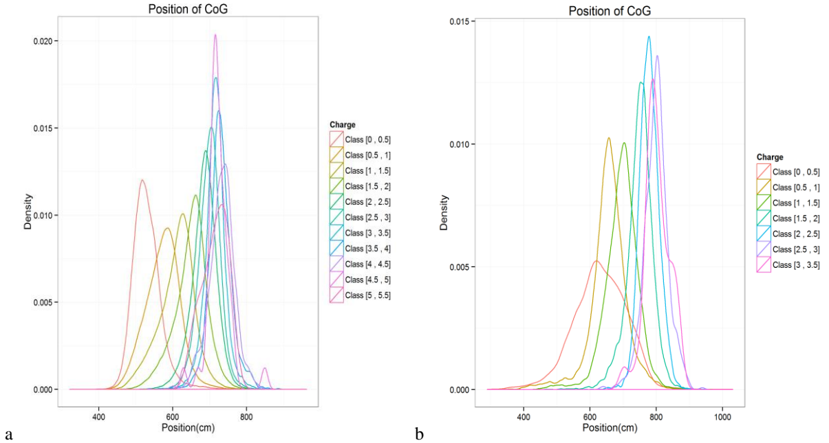
Fig. 4. Location of the payload CoG: (a) 5-axle articulated, (b) 2-axle rigid truck with a 2-axle trailer (on each diagram, the load classes are by 5 t step, e.g. class [0.5,1] contains the payload between 2.5 and 5 t).
