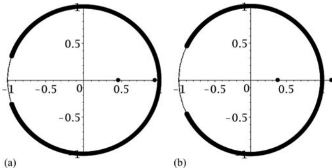
FIG. 4. Evolution of eigenvalues of the monodromy matrix corresponding to pitchfork bifurcation. N = 400 , a = 0.8 , k = 0.8 ; (a) \gamma = 0.05 , (b) \gamma = 0.045 .
