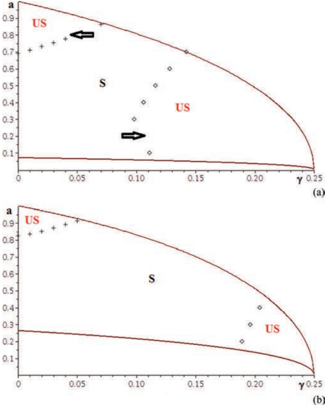
FIG. 2. (Color online) Zones of existence and stability for the symmetric DB on the (\gamma, a) parameter plane for two different values of the restitution coefficient: (a) k = 0.8 ; (b) k = 0.4 . Crosses denote the pitchfork bifurcation line and diamonds denote the line of Neimark-Sacker bifurcation. Transitions corresponding to illustrations in Figs. 2 and 3 are marked by arrows in (a). “S” and “US” denote zones of stability and instability, respectively.
