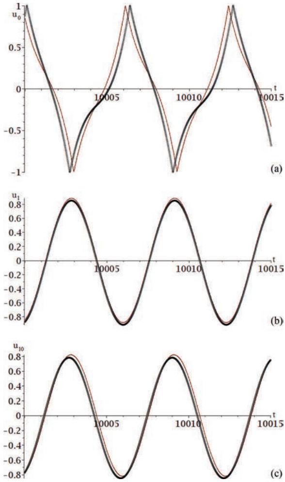
FIG. 7. (Color online) Comparison between exact solution for the symmetric DB in the infinite chain (12)-(13) (red, solid line) and numeric simulation of system (22) (black, circles) for N = 20 ; periodic boundary conditions, a = 0.82 , k = 0.8 , \gamma = 0.04 , and \mu = 0.005 . The time series are depicted for (a) u_0(t) ; (b) u_1(t) ; (c) u_{10}(t) .
