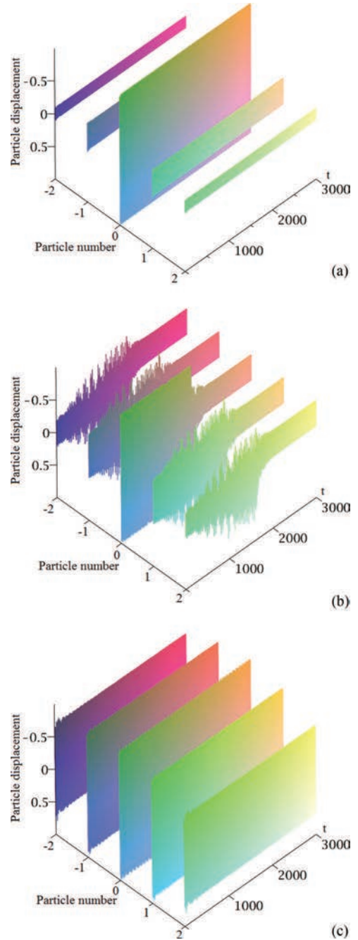
FIG. 6. (Color online) Numeric simulation of the DBs in small system with smoothed potentials and damping, N = 20 , k = 0.8 , \gamma = 0.104 ; (a) a = 0.1 , (b) a = 0.2 , (c) a = 0.7 . Time series for five central particles ( -2 \leq n \leq 2 ) are presented.
