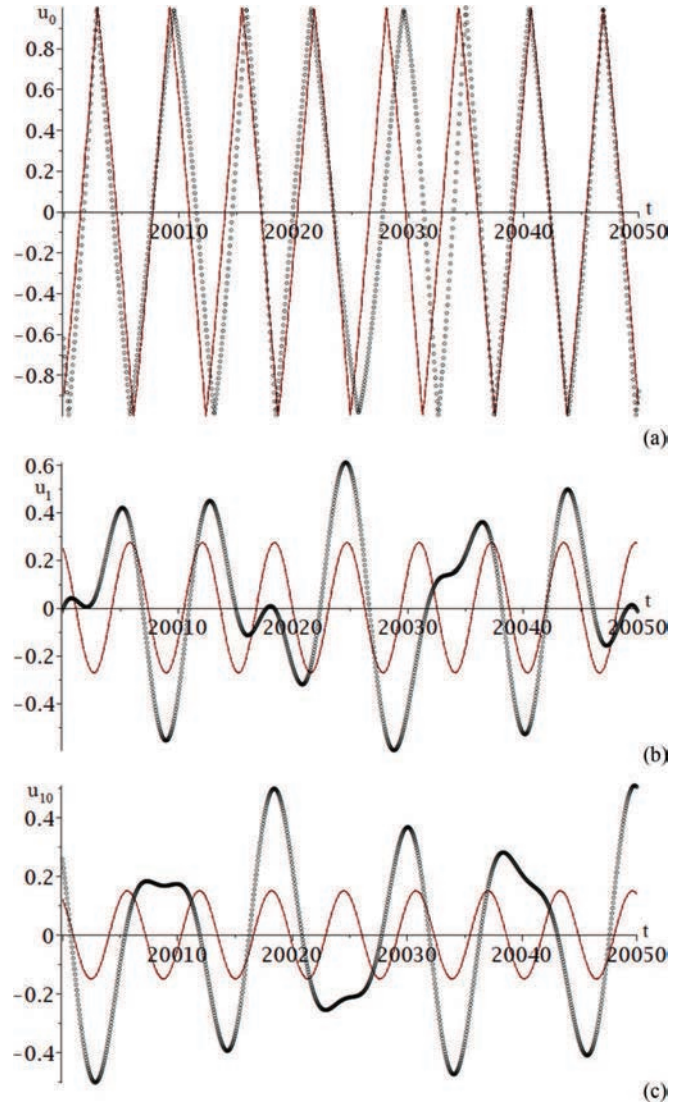
FIG. 8. (Color online) Comparison between exact solution for the symmetric DB in the infinite chain (12)-(13) (red, solid line) and numeric simulation of system (22) (black, circles) for N = 20 ; periodic boundary conditions, a = 0.15 , k = 0.8 , \gamma = 0.104 , and \mu = 0.005 . The time series are depicted for (a) u_0(t) ; (b) u_1(t) ; (c) u_{10}(t) .
