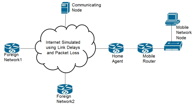
Fig. 1. Testbed implementation architecture
