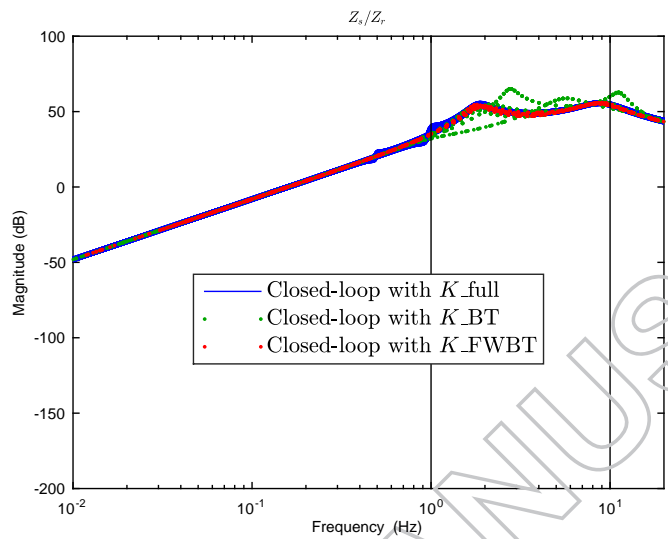
Figure 6.: Bode diagram magnitude of the transfer T_{\dot{z}_s/z_r}
