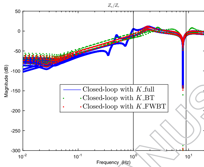
Figure 5.: Bode diagram magnitude of the transfer T_{z_s/z_r}
