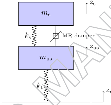
Figure 3.: Quarter-vehicle model
