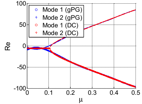
Fig. 13. Real parts of modes 1 and 2 ( r = 3 , p_{\text{optimal}} = 6 ).
