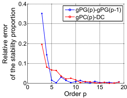
Fig. 12. Relative error of stability proportion.
