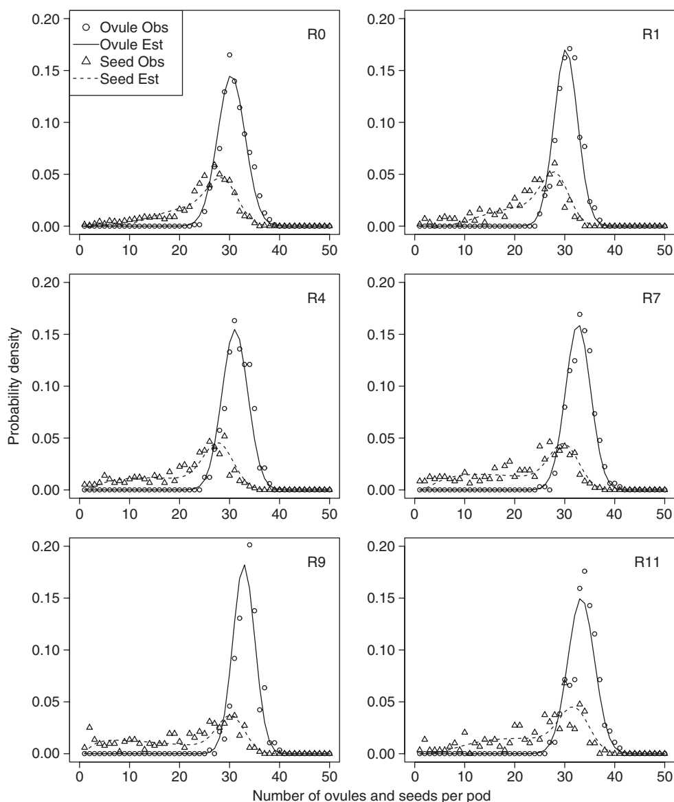
Figure 3 Estimated and observed number of ovules per flower and number of seeds per pod on the main stem R0 and for the 1st, 4th, 7th, 9th and 11th ramifications counting from the main stem apex (cv. Mendel). The symbols (Obs) and lines (Est) represent the observed and estimated values, respectively.
