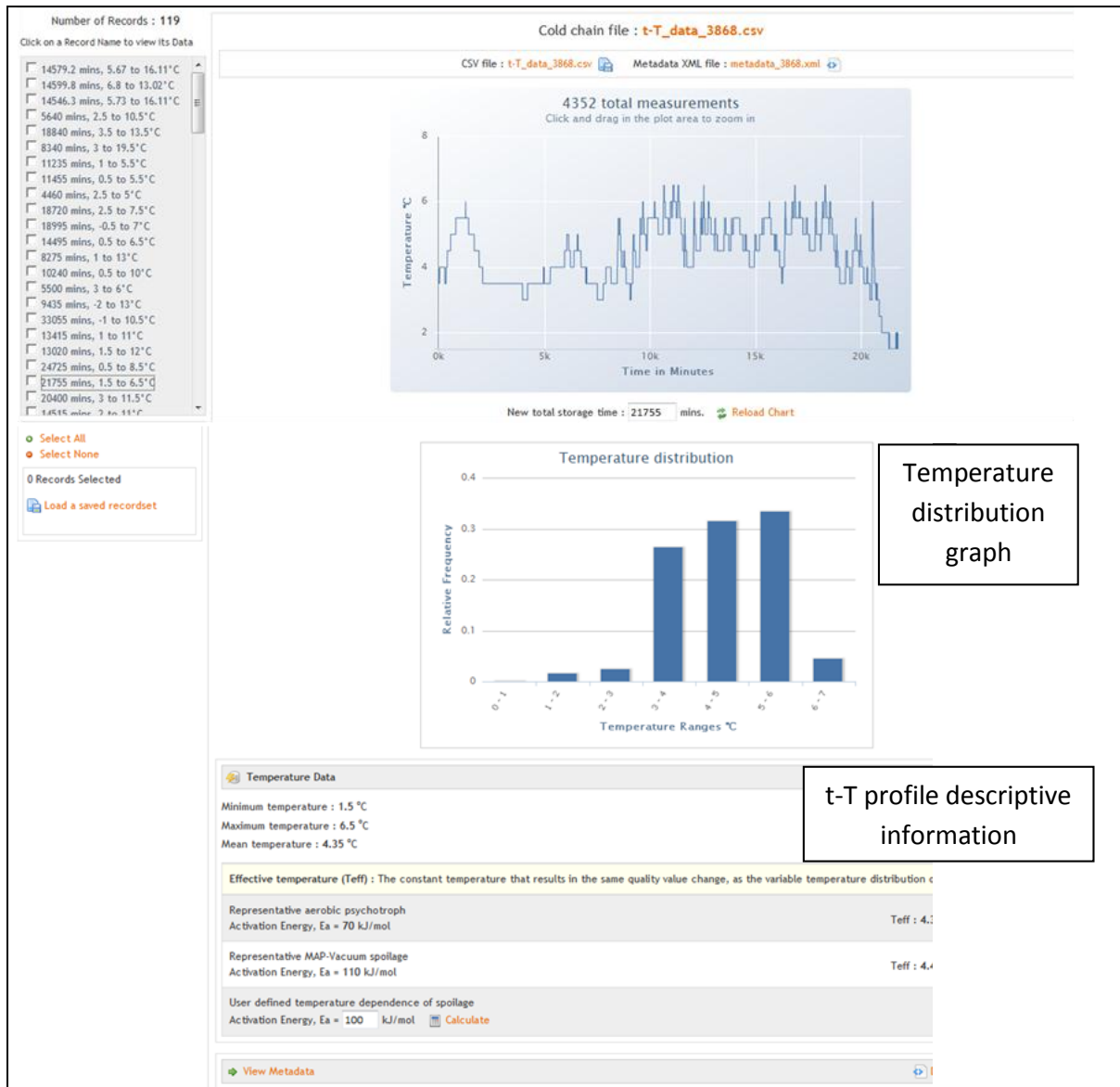
Pictue 2. Description of the Cold Chain Data Collection Platform output
