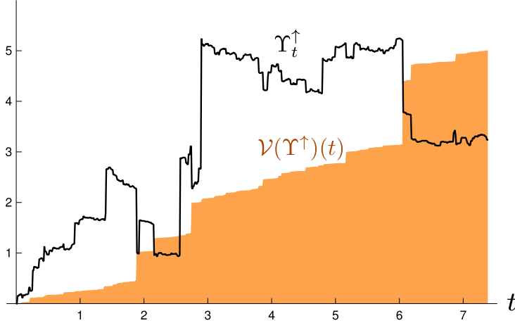
Figure 3: Simulation of the processes \Upsilon^\uparrow and \mathcal{V}(\Upsilon^\uparrow) .
