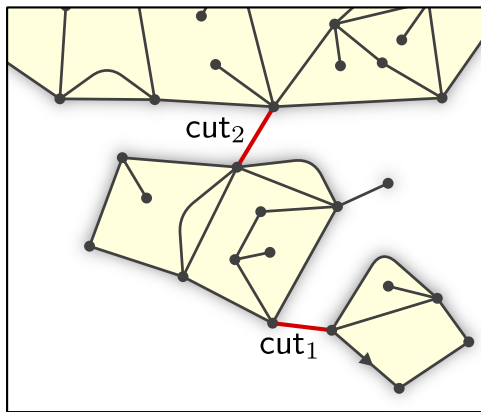
Figure 6: Illustration of the decomposition of \mathfrak{M}^{(\infty)} .
