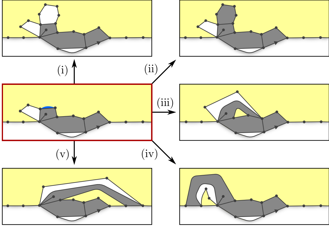
Figure 7: The map on the left in the red frame depicts an explored region satisfying hypothesis (H). The five other figures correspond to the five different situations when peeling the edge indicated in blue.
