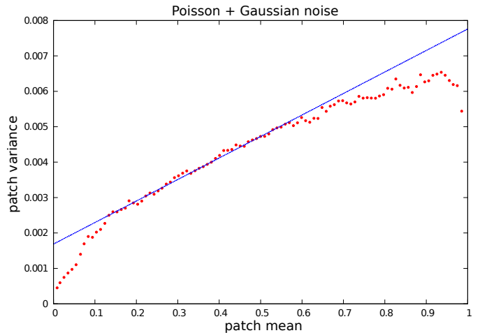
Figure 1. Patches variances according to the patch mean. The lower and higher pixel intensities are discarded. The line is fitted with RANSAC.
