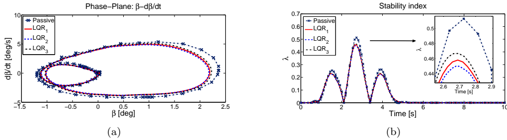
Figure 10. Phase-Plane \beta - \dot{\beta} (a) and Stability index \lambda (b).
