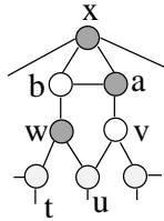
Figure 8: The case |X| = 3 .
