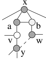
Figure 4: Vertex v , has a degree 4 neighbor y .
