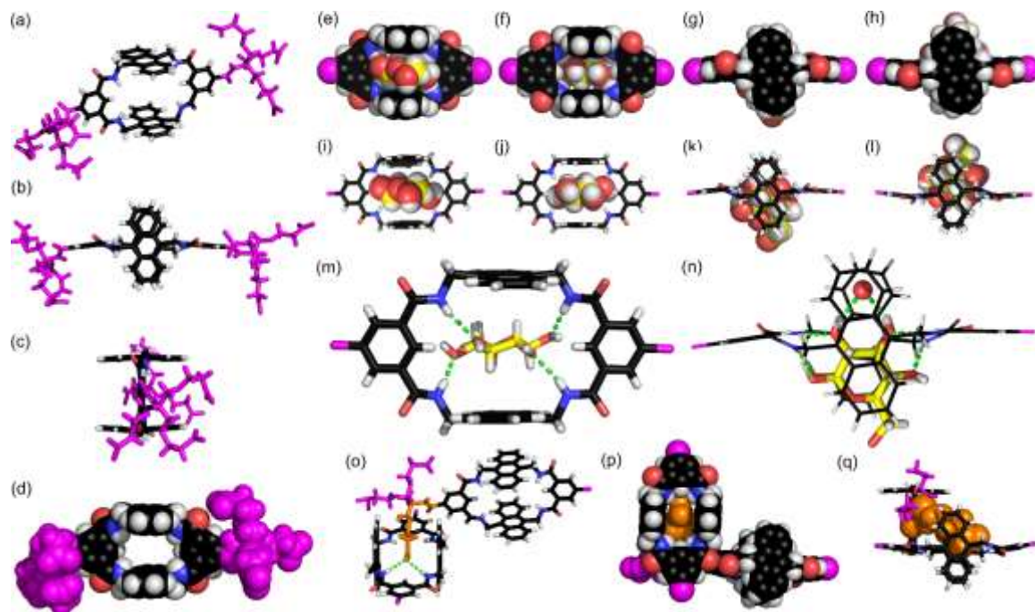
Fig. 3 Crystal structure of 1⊃2 . (a) front view, (b) top view, (c) side view, and (d) back view of macrocycle 1 shown in tube (a-c) or CPK (d) representations. The dendritic side chains are coloured in magenta. (e,i) front view, (f,j) back view, (g,k) top view and (h,l) bottom view of the structure of host-guest complex 1⊃2-D . The carbohydrate is shown in CPK representation in all cases whereas the macrocycle is shown either in CPK (e-h) or in tube (i-l) representations. Enlarged front (m) and top (n) views of 1⊃2-D in tube representation show the array of host-guest intermolecular hydrogen bonds. In (n) an additional water molecule sandwiched in between the two anthracenyl moieties of the receptor is involved in two interactions with glucose. In (e-n) the solubilizing side chains have been omitted for clarity. (o-q) Views of the macrocycle carboxylate side chain (orange) intercalated in the empty cavity a neighbour macrocycle.
