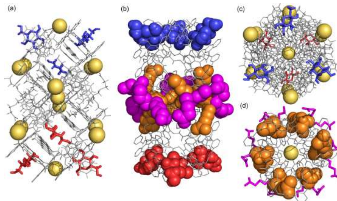
Fig. 2. Molecular packing in the crystal structure of 1 : 2 . (a) Side view of the dodecameric metallo-organic cluster of twelve molecules of 1 . The macrocycles are shown in light grey tube representation whereas D- \beta -glucopyranose and L- \beta -glucopyranose are coloured in blue and red, respectively. Some calcium cations are shown as gold CPK spheres. (b) Other view of the dodecameric cluster highlighting the insertion of some carboxylate side chains in the cavities of molecules of 1 that do not contain 2 . These chains are shown in orange CPK whereas other side chains are shown in magenta. Molecules of 2 are shown in CPK representation with the same color code as in (a). Calcium ions have been omitted for clarity. (c) Top view of the cluster showing the pseudo C_3 symmetry of the aggregate. (d) Top view of the six central macrocycles of the dodecamer ( i.e. peripheral macrocycles that host 2 have been removed) showing the arrangement of the intercalated carboxylate side chains. The side chains are coloured as in (b).
