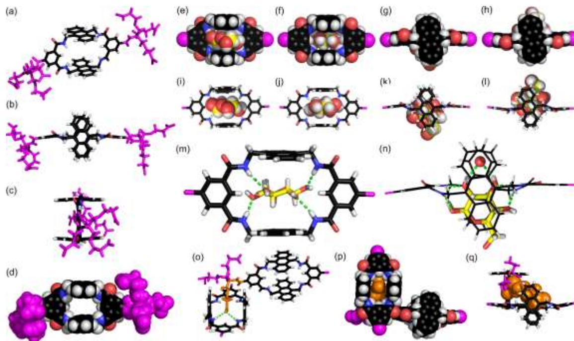
Fig. 3 Crystal structure of 1\supset 2 . (a) front view, (b) top view, (c) side view, and (d) back view of macrocycle 1 shown in tube (a-c) or CPK (d) representations. The dendritic side chains are coloured in magenta. (e,i) front view, (f,j) back view, (g,k) top view and (h,l) bottom view of the structure of host-guest complex 1\supset 2\text{-D} . The carbohydrate is shown in CPK representation in all cases whereas the macrocycle is shown either in CPK (e-h) or in tube (i-l) representations. Enlarged front (m) and top (n) views of 1\supset 2\text{-D} in tube representation show the array of host-guest intermolecular hydrogen bonds. In (n) an additional water molecule sandwiched in between the two anthracenyl moieties of the receptor is involved in two interactions with glucose. In (e-n) the solubilizing side chains have been omitted for clarity. (o-q) Views of the macrocycle carboxylate side chain (orange) intercalated in the empty cavity a neighbour macrocycle.
