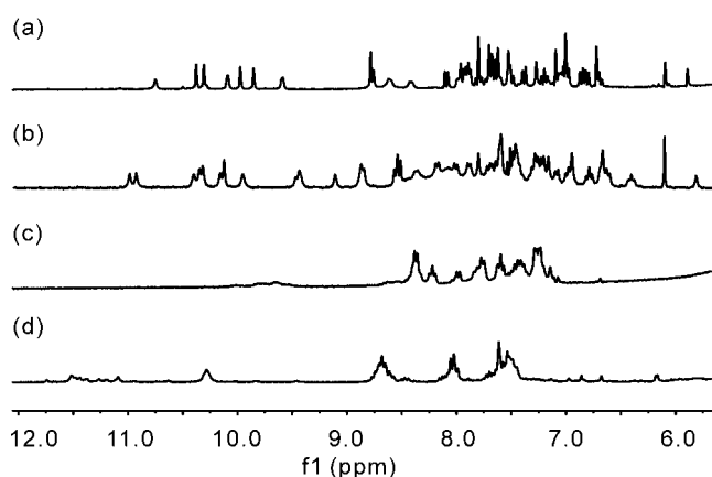
Figure 6. Part of the ^1\text{H} NMR spectra (300 MHz) of 10 and 11 showing aromatic amide (9 – 12 ppm), aliphatic amide and aromatic proton resonances (6 – 10 ppm) in protic solvents at 25°C: (a) 11 in \text{H}_2\text{O}/\text{D}_2\text{O} (9:1 v/v); (b) 11 in \text{MeOH-d}_3 ; (c) 10 in \text{H}_2\text{O}/\text{D}_2\text{O} (9:1 v/v); (d) 10 in \text{MeOH-d}_3 .
