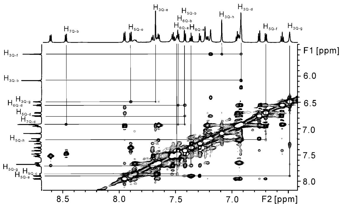
Figure 9. Excerpt from NOESY spectrum of 12 in D 2 O at 25°C (800 MHz) showing the NOE correlations between aromatic protons of quinolines at i and i + 3 .
