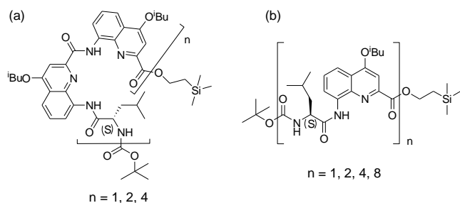
Figure 1. Structures of (a) LQ^{Leu_2} and (b) LQ^{Leu} -type sequences.
