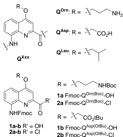
Figure 2. Structures of Q^{Xxx} and Fmoc-protected quinoline monomers.
