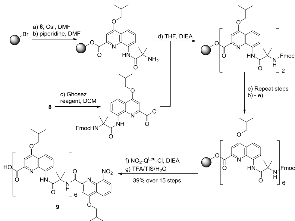
Scheme 3. SPS of the 13mer 9 from the dimeric unit 8 .
