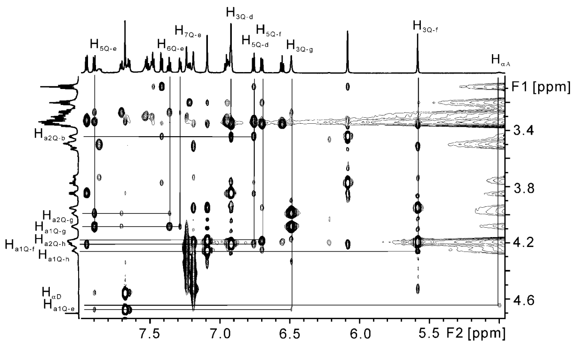
Figure 10. Excerpt from NOESY spectrum of 12 in D 2 O at 25°C (800 MHz) showing the NOE correlations between quinoline side-chain methylene protons and aromatic protons of quinolines at i + 3 .
