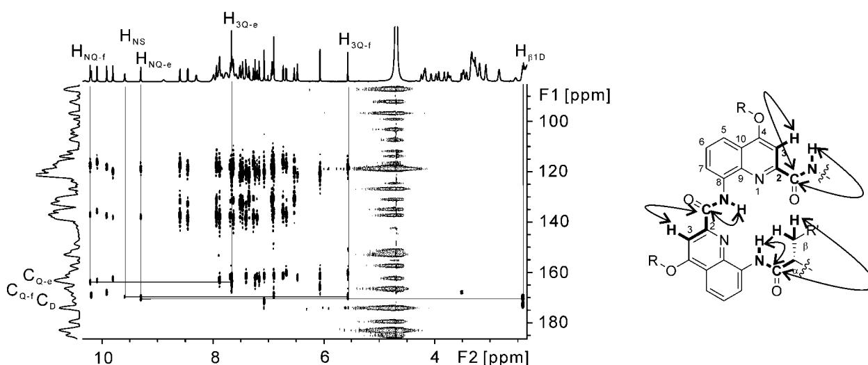
Figure 8. Excerpt from HMBC spectrum of 12 in H_2O/D_2O (9:1 v/v) at 25^\circ C (700 MHz) indicating the correlations involved in assigning the –DQQS- fragment of the sequence. Double-headed arrows indicate the observed correlations.
