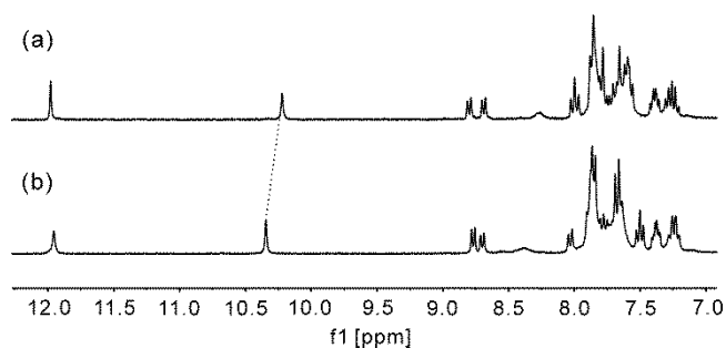
Figure 4. The amide and aromatic region of 1 H NMR spectra (300 MHz) of crude (a) 4b and (b) 5b in DMSO-d 6 showing a single set of signals in each instance.
