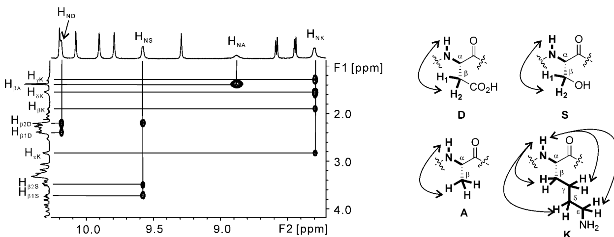
Figure 7. Excerpt from TOCSY spectrum of 12 in \text{H}_2\text{O}/\text{D}_2\text{O} (9:1 v/v) at 25°C (700 MHz) indicating the correlations between aliphatic amide proton ( \text{H}_{\text{NX}} ) and side-chain methylene protons ( \text{H}_{\text{X}} ) of each amino acid. Double-headed arrows indicate the observed correlations.
