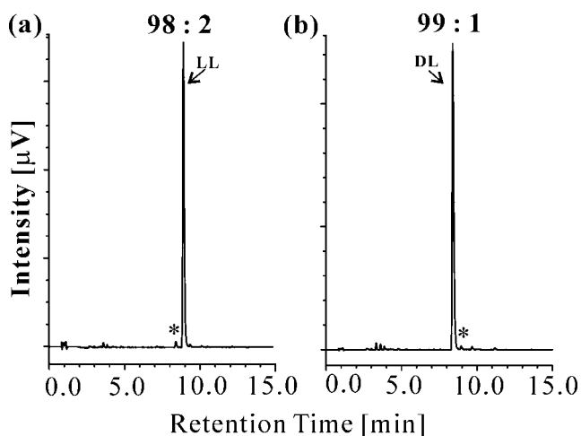
Figure 3. RP-HPLC chromatogram of crude products (a) 4a and (b) 5a . LL = Fmoc-Ala-Ala-(Q) 2 -OH, DL = Fmoc-DAla-Ala-(Q) 2 -OH; * = putative by-product of racemization during in-situ acid chloride coupling.
