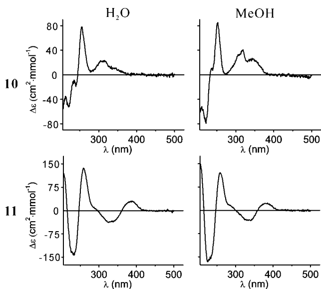
Figure 5. CD spectra of 10 and 11 in H 2 O and MeOH. (Concentration: 30 μM)
