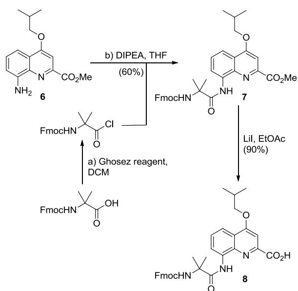
Scheme 2. Synthesis of the Fmoc-AiB-Q Leu -OH dimer building block 8 .
