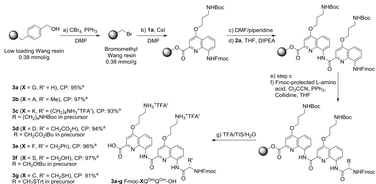
Scheme 1. Solid phase synthesis of various Fmoc- XQ_2 -OH hybrid tripeptides.
