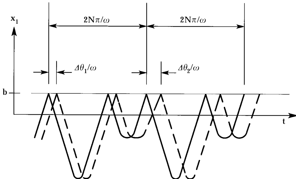
Figure 2. Local stability analysis.
