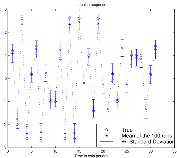
Fig. 9 : Monte Carlo results on estimated impulse response
