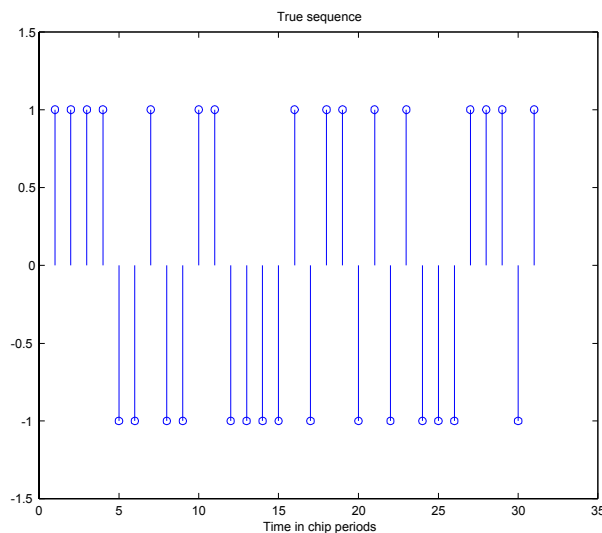
Fig. 2 : Gold sequence
