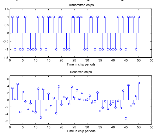
Fig. 8 : Transmitted and Received chips
