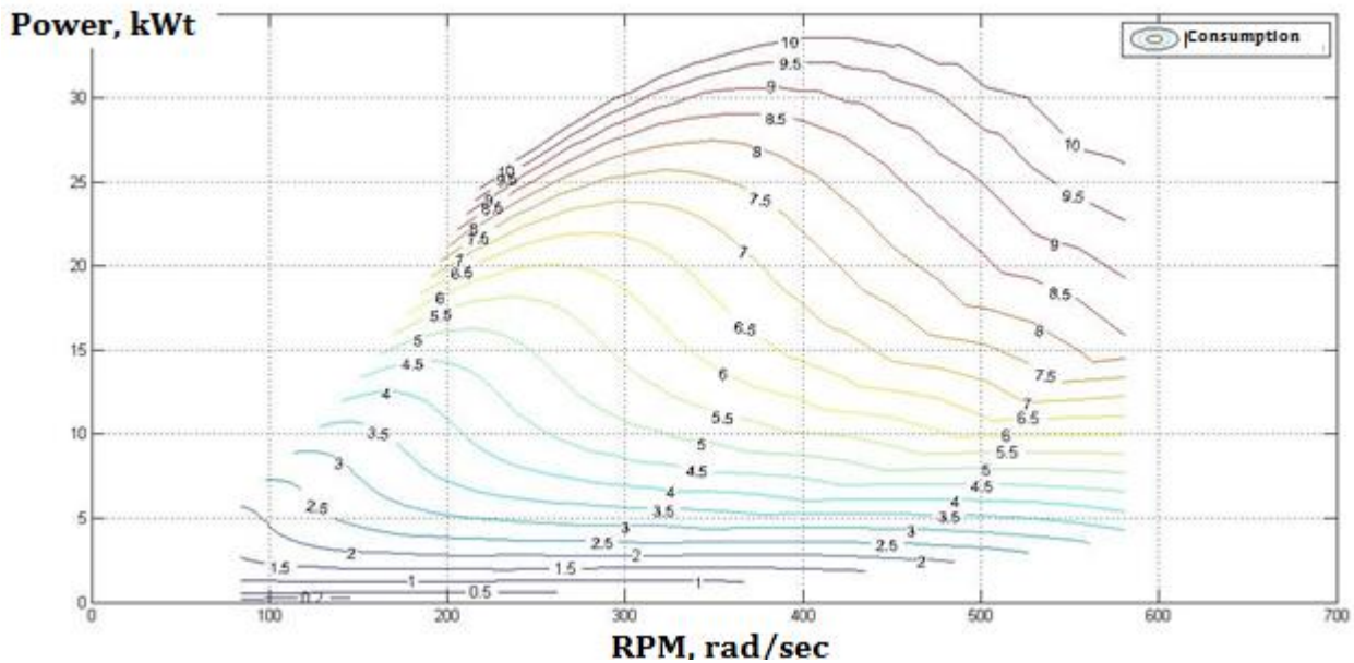
Fig. 13. Fuel consumption.
