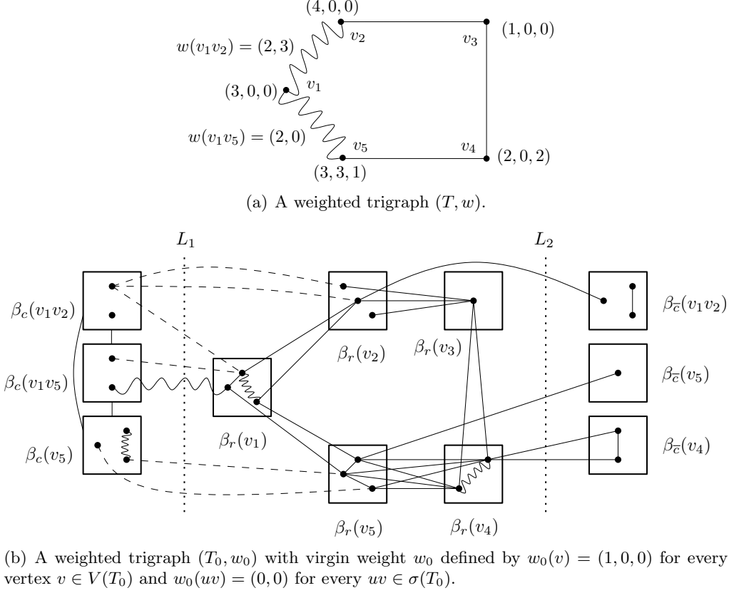
Figure 4: Illustration for the definition of a model: the weighted trigraph (T, w) depicted in (a) is a model of the weighted trigraph (T_0, w_0) depicted in (b), as witnessed by the partition map \beta (empty teams are not depicted). Each vertex at the left-hand-side of dotted line L_1 is assumed to be strongly adjacent to every other vertex except if a non-edge is explicitly drawn (with a dashed edge for strong antiedge and with a wiggly edge for a switchable pair). Similarly, each vertex at the right-hand-side of dotted line L_2 is assumed to be strongly antiadjacent to every other vertex except if an edge is explicitly drawn.
