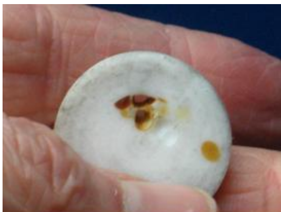
Figure 19: Enhanced electronic sputtering of insulators. PTFE disc, 5mm thick. Irradiated with \sim 1 MeV protons in \sim 1993-4 to do machine calibration using the resonant \text{F}(p, \gamma) reaction at 990 keV for work reported in (Kazor et al. 1994)
