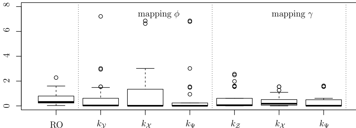
Fig. 3: Optimality gap for the Branin test function with d = 2 and D = 25 with a budget of one hundred evaluations over 25 runs. The domains for the mapping \phi and \gamma are \mathcal{Y} = [-\sqrt{d}, \sqrt{d}]^d and \mathcal{B} respectively
