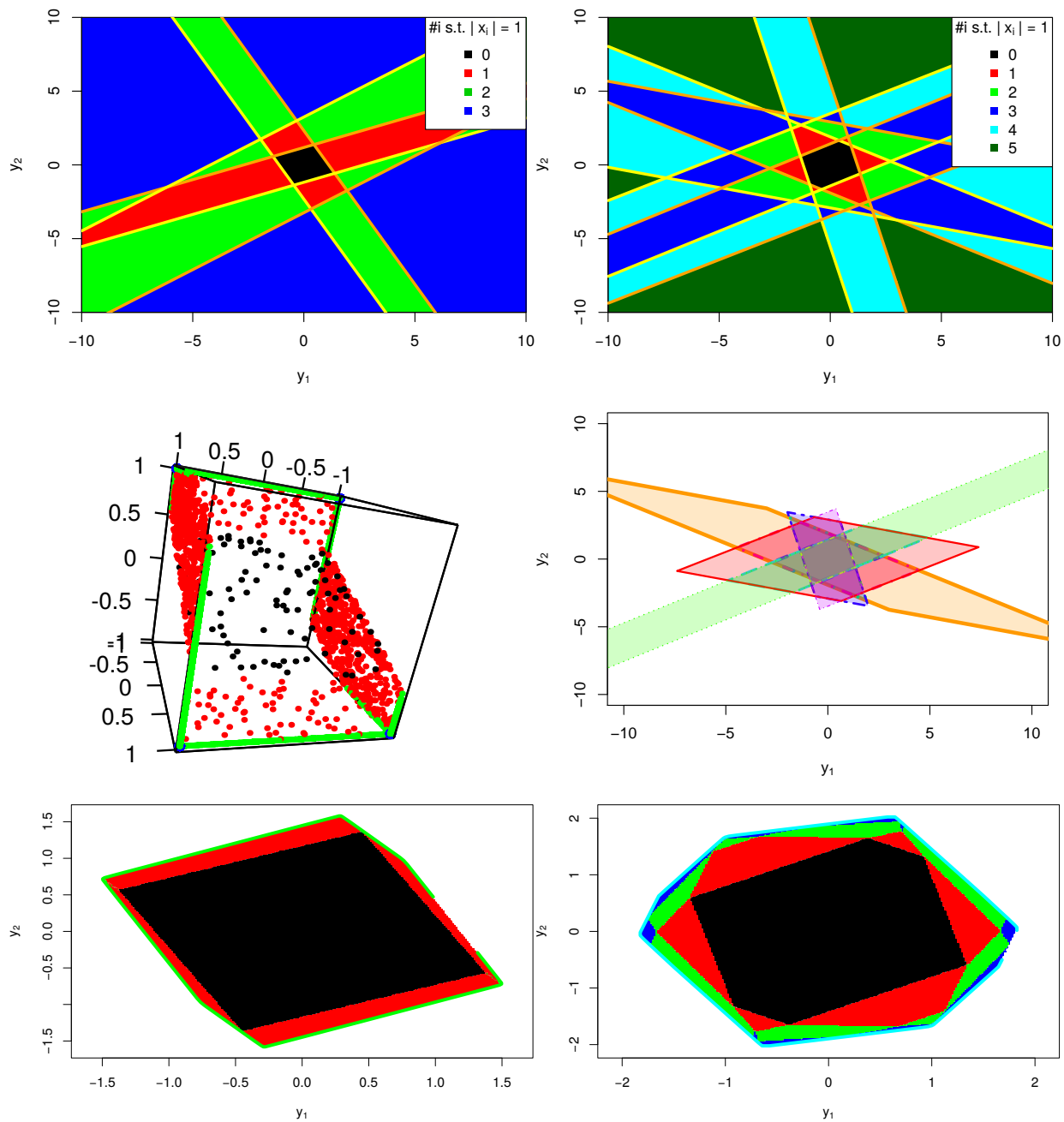
Fig. 2: Representation of the sets of interest introduced in Section 2 with d = 2 and D = 3 (left) or D = 5 (right) in \mathcal{Y} with \phi (top and center right), in \mathcal{X} (center left) and in \mathcal{Y} with \gamma (bottom). Except for the right center panel, colors represents how many variables in \mathcal{X} are not in ] - 1, 1[ . Top: the orange and yellow lines are the parallel hyperplanes forming the strips \mathcal{S}_i . The intersection of all parallelograms \mathcal{I} is in black. Center right: each of the 10 parallelotopes (here parallelograms) \mathcal{P}_I is depicted with a different color and their union is the minimal set \mathcal{U} . For illustration purpose, \mathcal{U} is truncated: the green cut parallelogram is approximately enclosed in [-210, 210] \times [130, 130] . Bottom: the different colored sets form zonotopes \mathcal{Z} .
