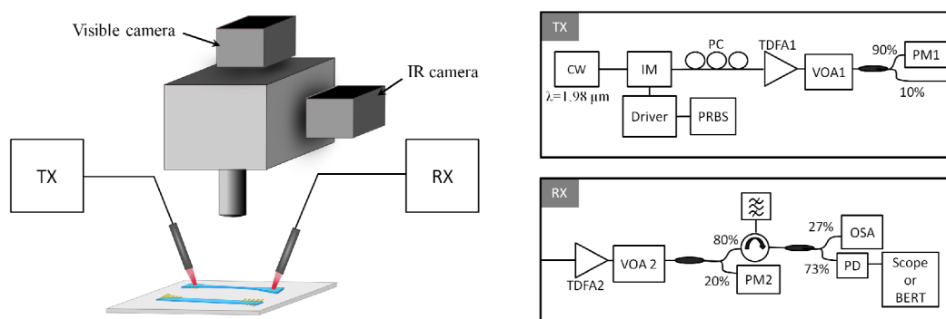
Figure 5. Experimental setup for a 10-Gbit/s 2-μm optical transmission. CW: continuous wave; IM: intensity modulator; PC: polarization controller; PRBS: pseudorandom binary sequence; TDFA: thulium-doped fiber amplifier; VOA: variable optical attenuator; PM: power meter; OSA: optical spectrum analyzer; PD: photodiode; BERT: bit error rate tester (model MU181040A, Anritsu Corporation, Atsugi-shi, Japan).
