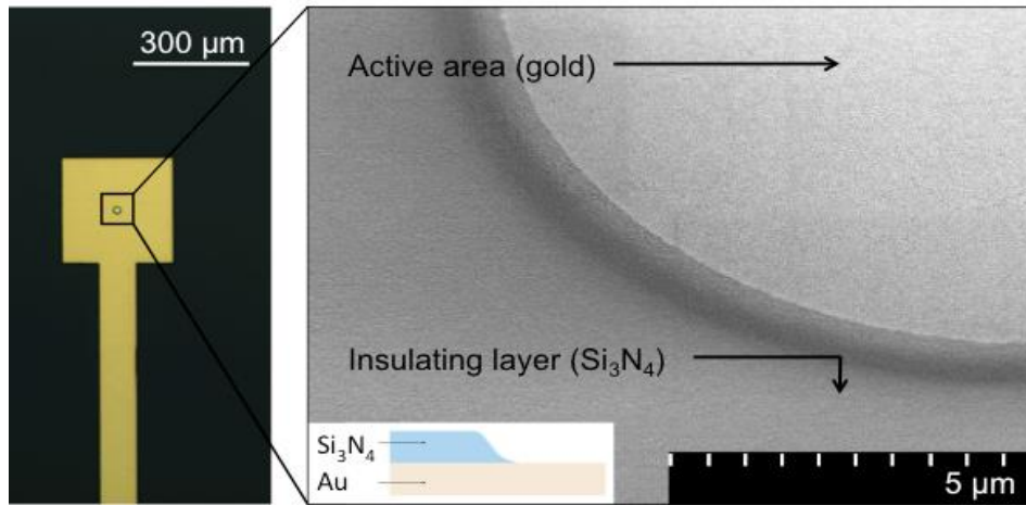
Figure 2: Microscope image and (insert) SEM image of a typical gold microelectrode
