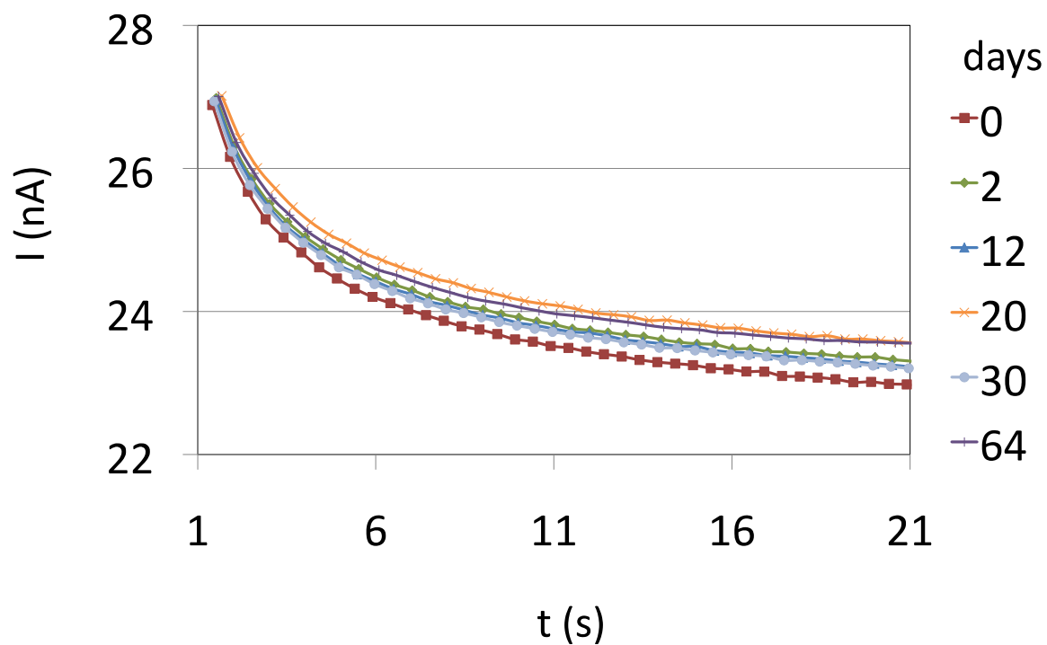
Figure 4: Temporal evolution of chronoamperometric curves
