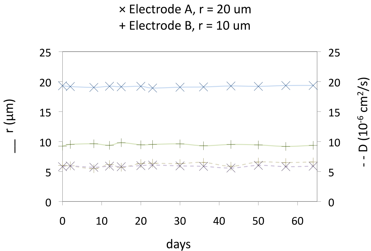
Figure 6: Temporal evolution of microelectrode electroactive surface radius r and of \text{Fe}(\text{CN}_6)^{4-} diffusion coefficient D test values during ageing in natural seawater
