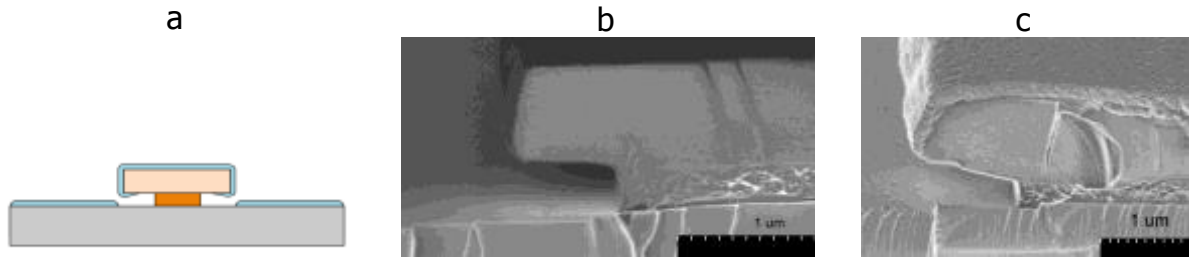
Figure 1: Silicon nitride deposition on T-shaped bilayer resist (a), SEM images of the T-shaped bilayer resist profile (b) before and (c) after the SiN x film deposition
