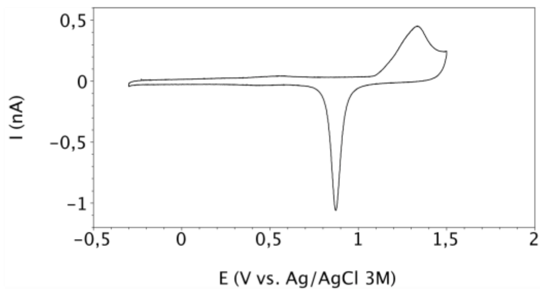
Figure 3: Gold microelectrode ( r = 10 \mu\text{m} ) cyclic voltammogram in a deaerated 0.5 \text{ M H}_2\text{SO}_4 solution (potential scan rate: 50 \text{ mV/s} )
