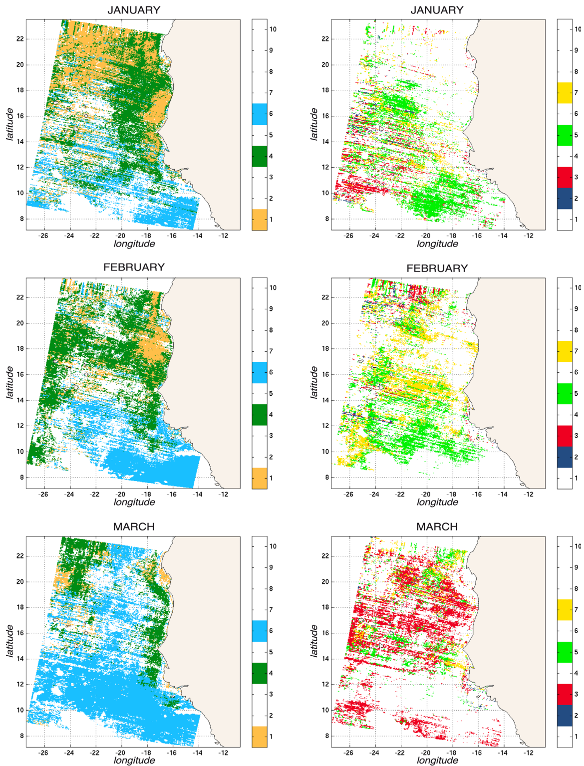
Figure 7b. The 13 year climatology of the classes for January, February, and March. (left) We have represented class-1 (orange), class-4 (green), and class-6 (light blue). (right) We have represented class-2 (blue), class-3 (red), class-5 (light green), and class-7 (yellow).
