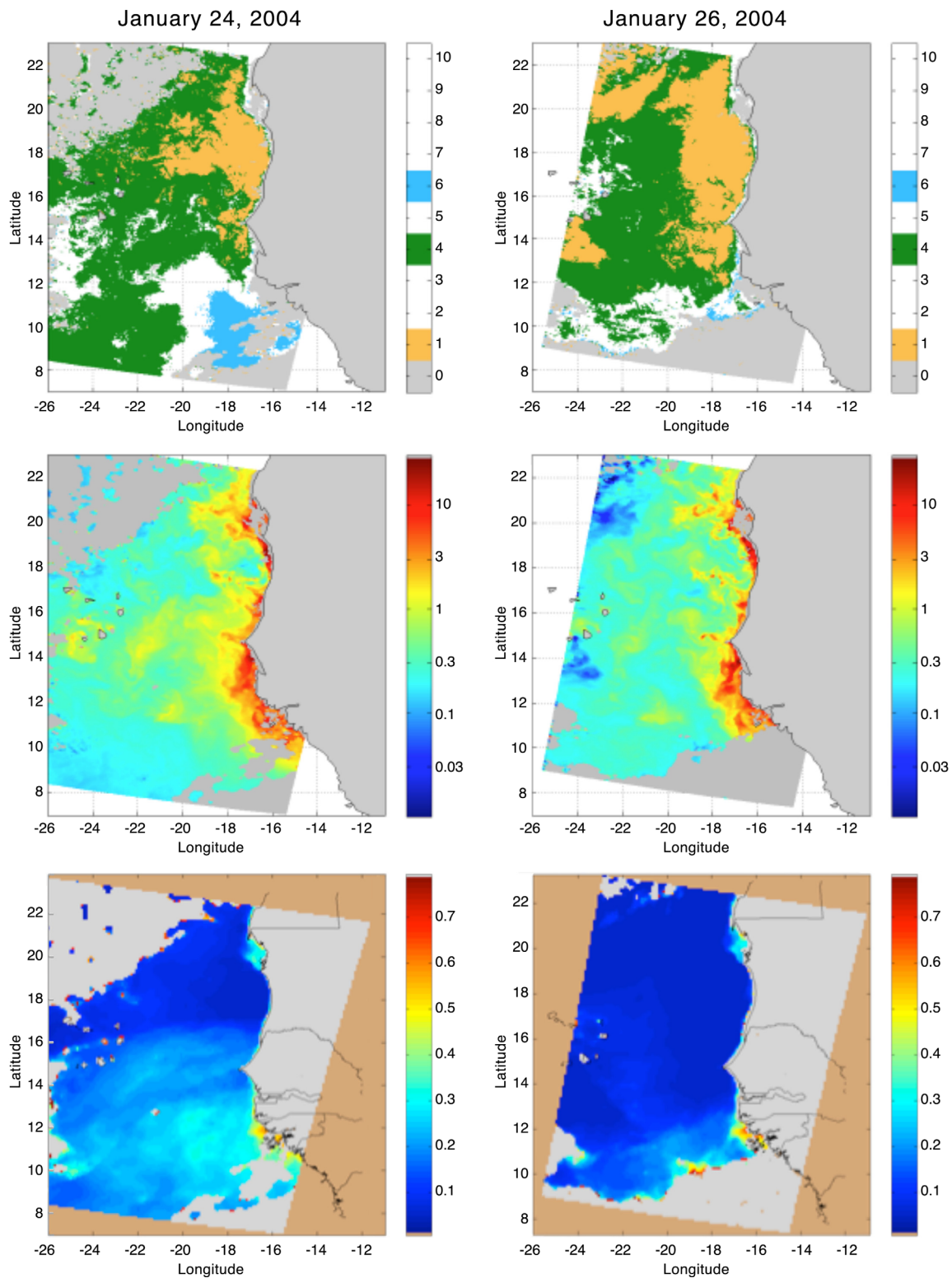
Figure 9b. (top) Spectrum pattern of class-1, class-4, and class-6, (middle) the associated chlorophyll- a concentration, and (bottom) AOT for the 24 and 26 January 2004, days for which AOT coverage was very low. Class-1 (haptophytes) is in orange, class-4 ( Prochlorococcus ) in green, and class-6 (SLC) in light blue. AOT low values are in blue.
