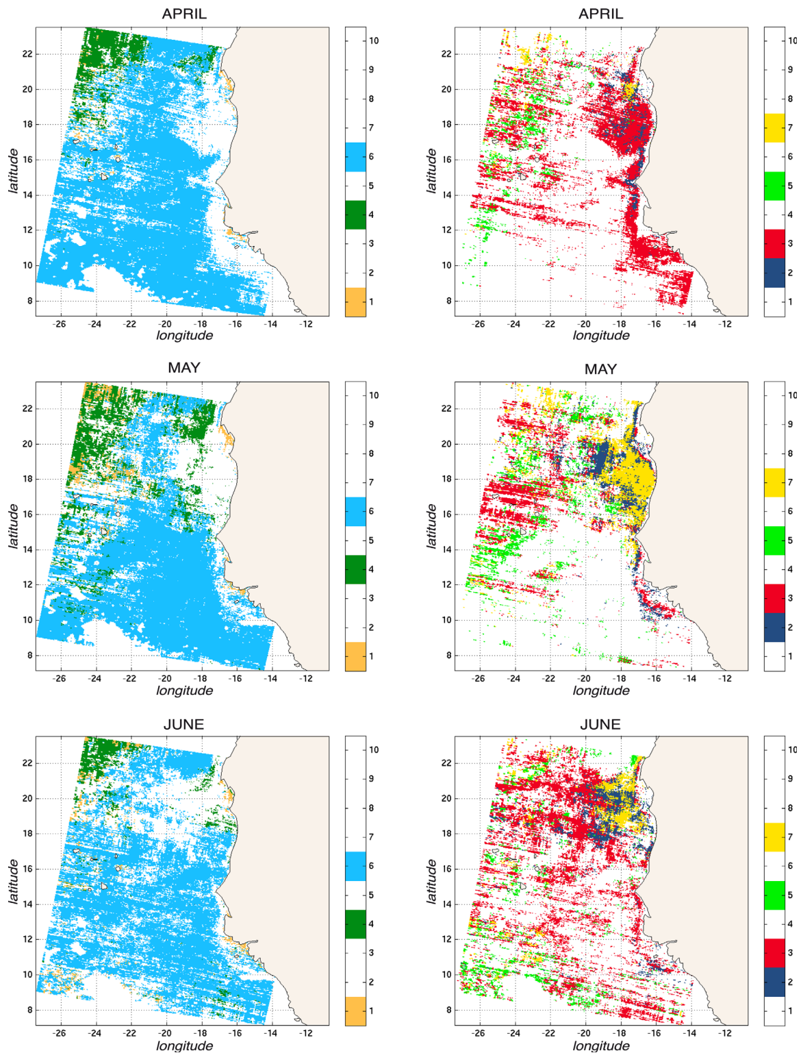
Figure 7c. The 13 year climatology of the classes for April, May, and June. (left) We have represented class-1 (orange), class-4 (green), and class-6 (light blue). (right) We have represented class-2 (blue), class-3 (red), class-5 (light green), and class-7 (yellow).
