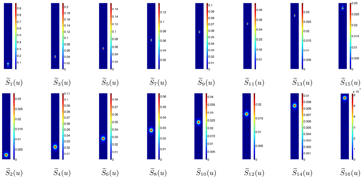
FIGURE 8. Sensitivity indices \tilde{S}_i(u) of multiscale solution u with respect to each random variable \xi_i , i \in \{1, \dots, 16\} , where the first row gathers the sensitivity indices \tilde{S}_{2q-1}(u) associated with random diffusion coefficient K_q (parameterized by \xi_{2q-1} ) and the second row gathers the sensitivity indices \tilde{S}_{2q}(u) associated with random reaction parameter R_q (parameterized by \xi_{2q} ), q \in \{1, \dots, 8\}
