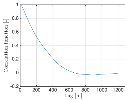
Figure 9. Correlation function of design horizontal curvature.
