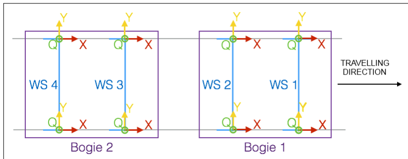
Figure 19. Measurement vehicle schema.
