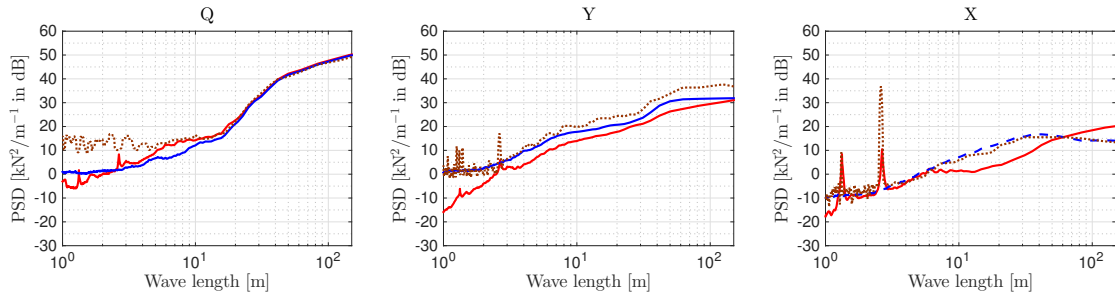
Figure 29. PSD of contact forces, front wheelset in alignment, constant velocity. Experimental data (red line), numerical simulations with track geometry irregularities without (dashed blue line) and with (dotted brown line) wheel untrueness.
