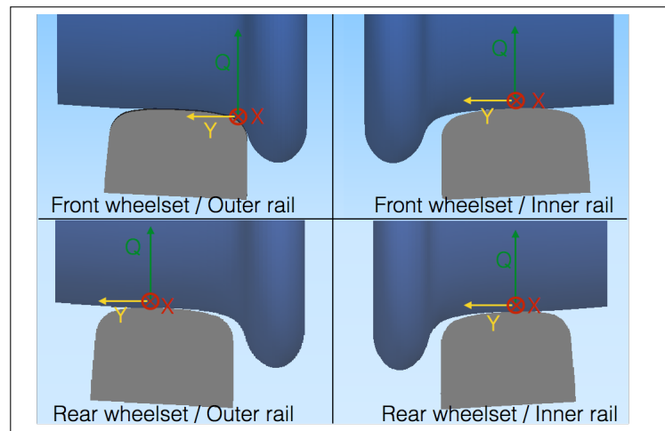
Figure 22. Example of contact positions in a curved track
