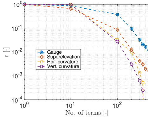
Figure 31. Evaluation of the quantity r , defined in Equation 28, for different numbers of Karhunen-Loève terms and for each generated field.
