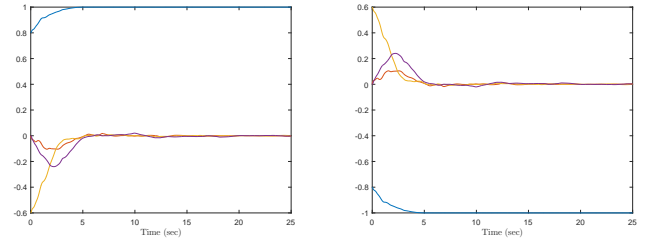
Fig. 1: Unit-quaternion tracking error \tilde{Q} for Test1 and Test2
