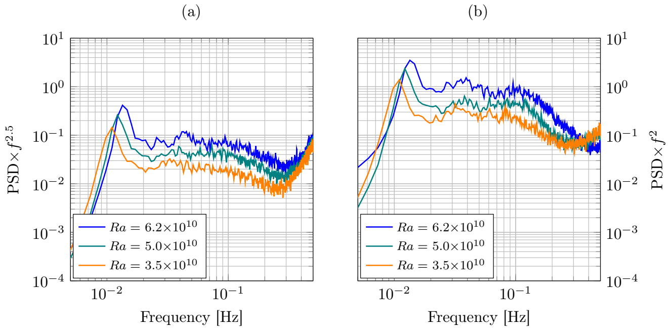
Figure 13: (a) Horizontal and (b) vertical velocity spectra compensated by f^{-2.5} and f^{-2} respectively for different Rayleigh numbers.
