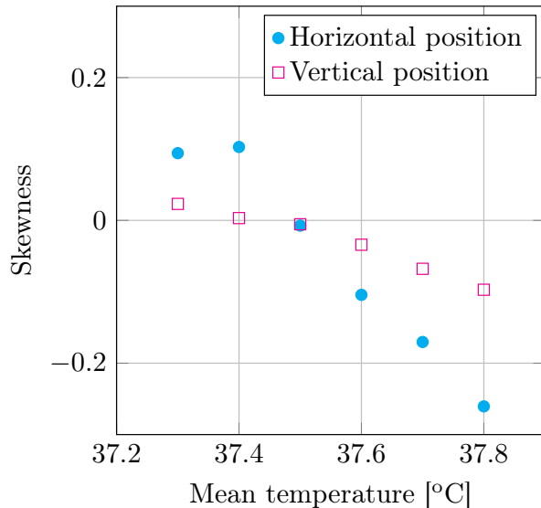
Figure 3: Skewness of the distribution of the vertical and horizontal positions of the smart particle versus the temperature of the cell center.
