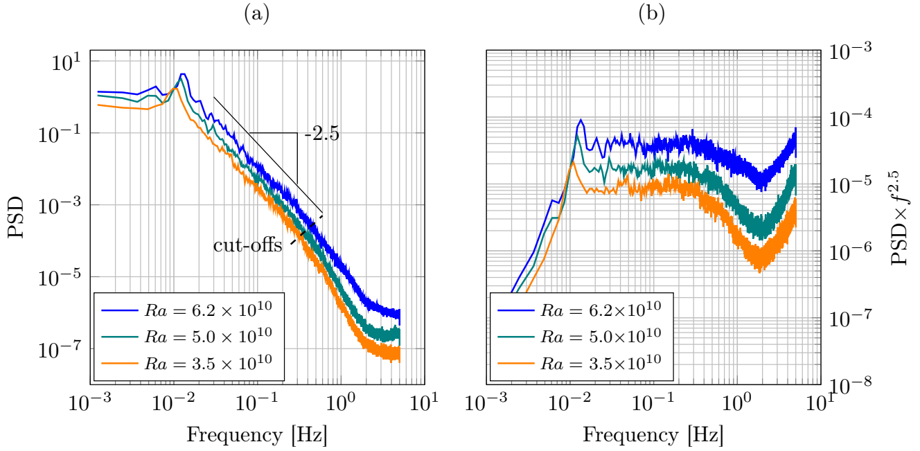
Figure 12: (a) Temperature spectra at different Rayleigh numbers. (b) Same temperature spectra compensated by f^{-2.5} .
