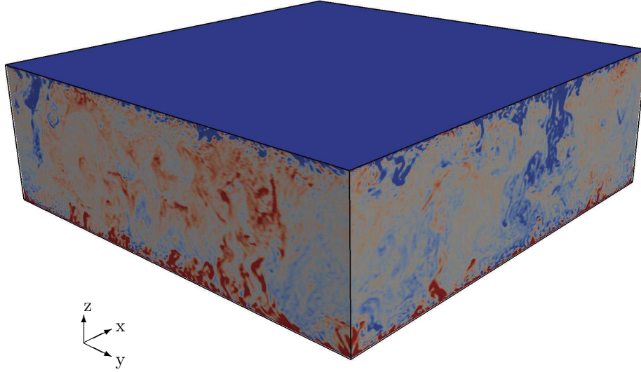
Figure 2: Sketch of the numerical simulation domain. Temperature contours for Ra = 10^9 are also shown (red indicates regions of high temperature whereas blue indicates regions of low temperature).
