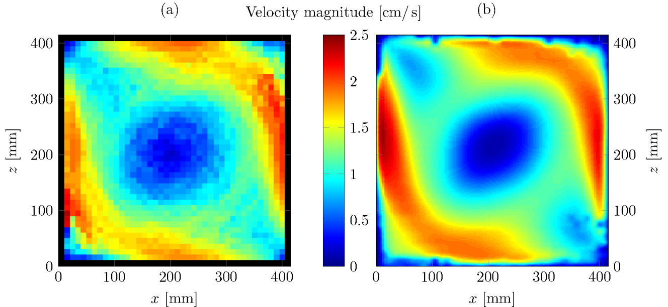
Figure 5: (a) Pseudo-Eulerian field of the velocity magnitude from Lagrangian data, Ra = 5.0 \times 10^{10} . (b) Field of the velocity magnitude obtained by PIV, Ra = 5.6 \times 10^{10} .
