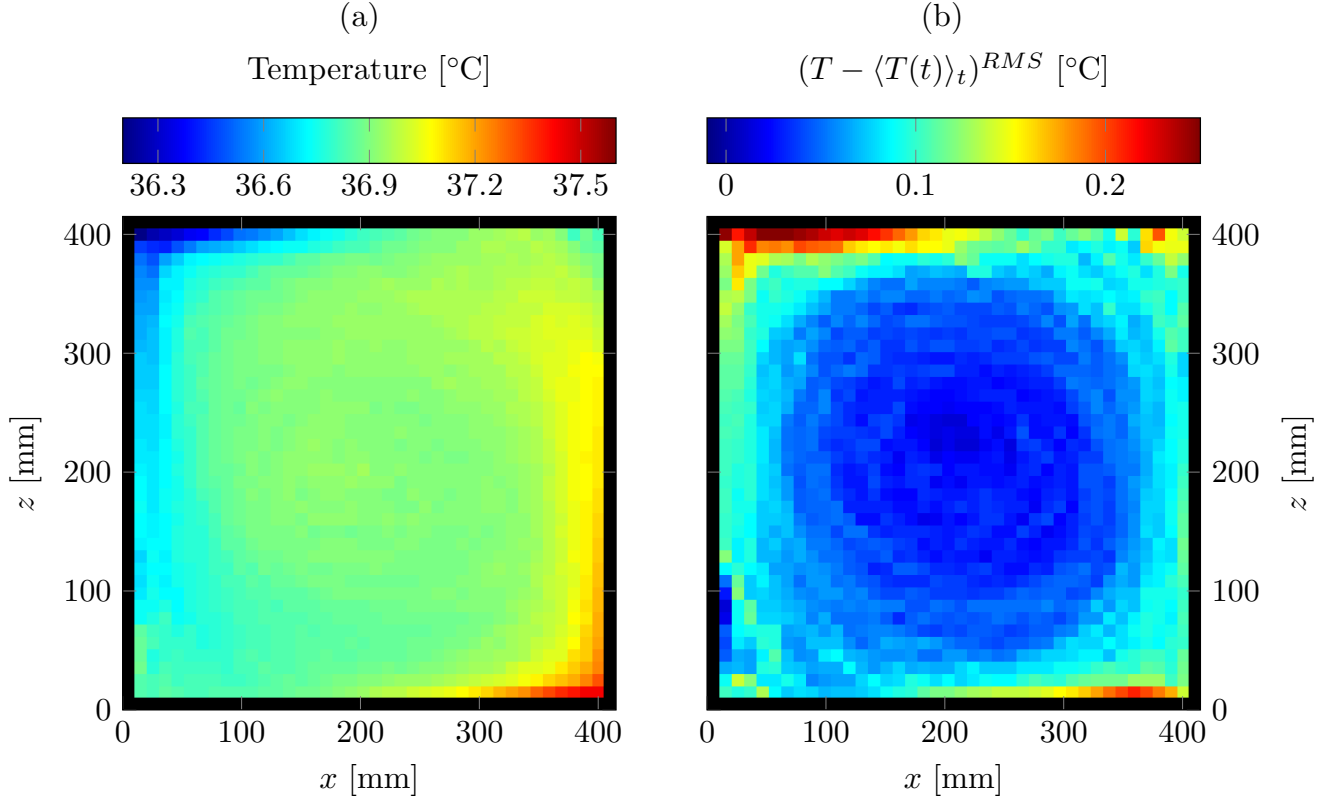
Figure 6: Pseudo-Eulerian (a) temperature field and (b) square mean root of the difference between the temperature and the temperature average along the trajectory. Measurements at Ra = 5.0 \times 10^{10} .
