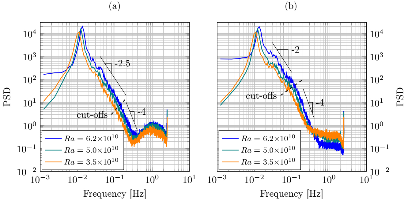
Figure 11: (a) Horizontal and (b) vertical velocity spectra at different Rayleigh numbers.
