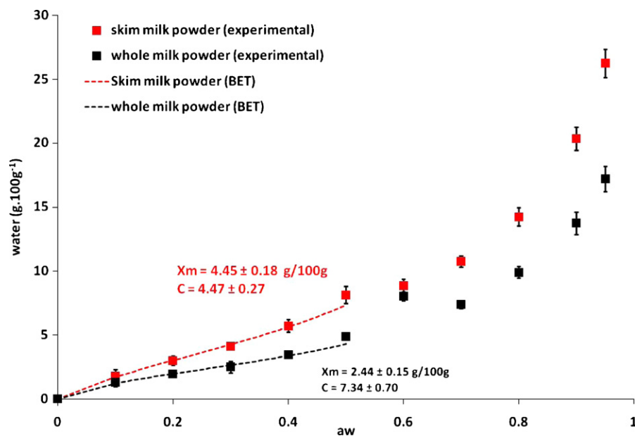
Fig. 7. Experimental and predicted water vapor sorption isotherms (mean of three independent analyses). Determination of the monolayer moisture content ( X_m ) and constant C with the BET model for relative humidity ranging between 0% and 50%.
