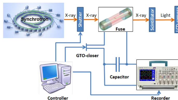
Figure 4: Simplified organization of the test equipment, showing its principal parts
