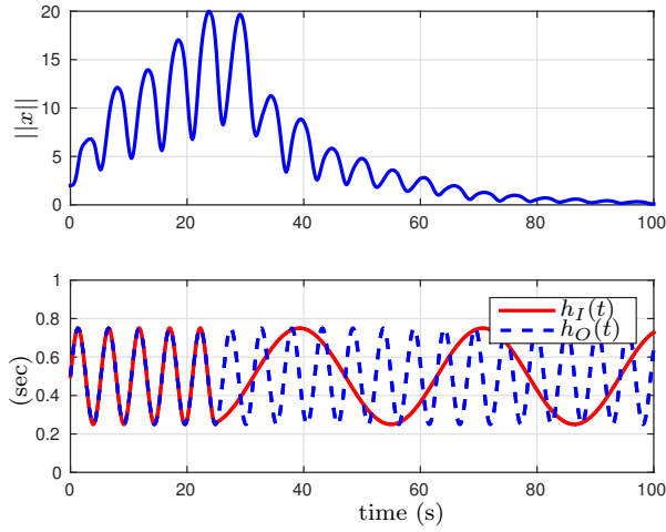
Figure 2. Top: Norm of the state – Bottom: Exact delay h(t) with different dynamics.
