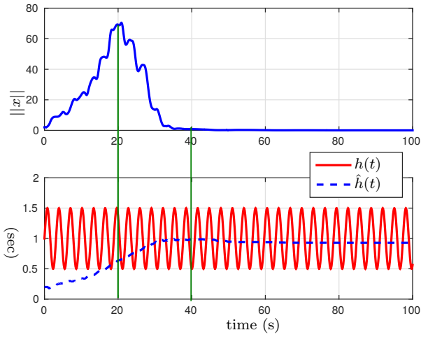
Figure 3. Top: Norm of the state – Bottom: Round trip delay h(t) = h_I(t) + h_O(t) and its estimation \hat{h}(t) from delay estimator in Léchappé et al. (2016).
