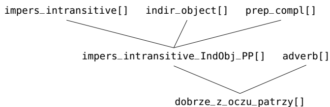
Figure 6: Inheritance hierarchy of the XMG classes in Figure 5
