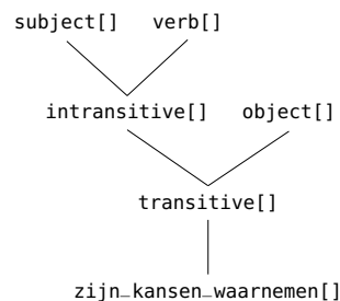
Figure 3: Inheritance hierarchy of XMG classes according to the code in Figure 2
