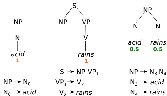
Figure 1: A toy LTAG grammar and its conversion into flat rules
