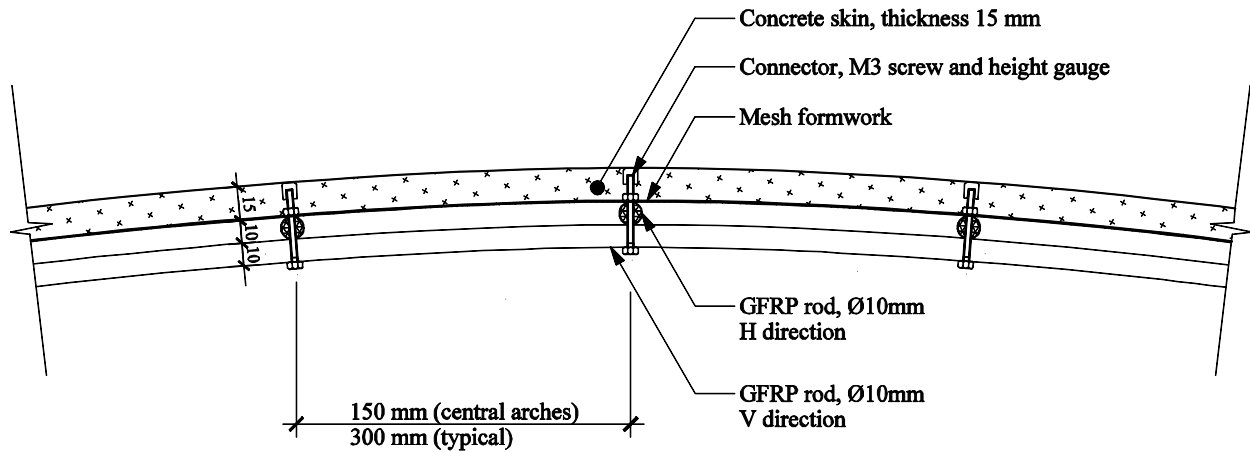
Figure 6: Section cut, typical.
