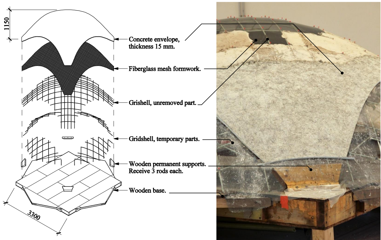
Figure 5: Axonometric view and photograph showing the successive layers in the prototype.
