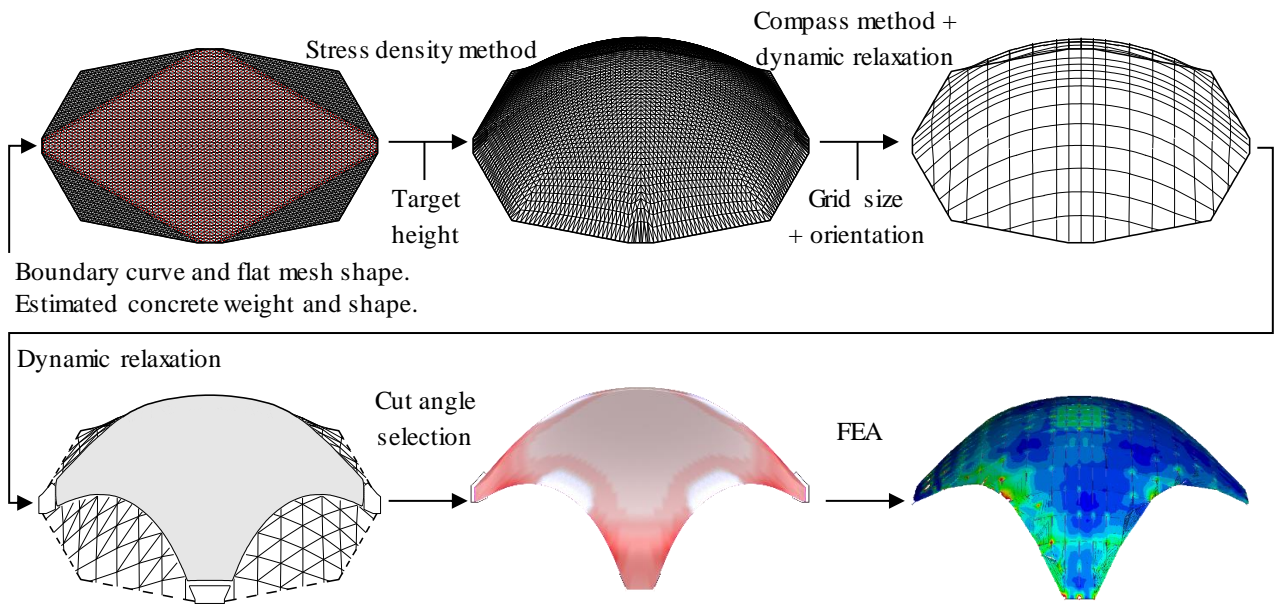
Figure 4: Steps of the design process used for the prototype.
