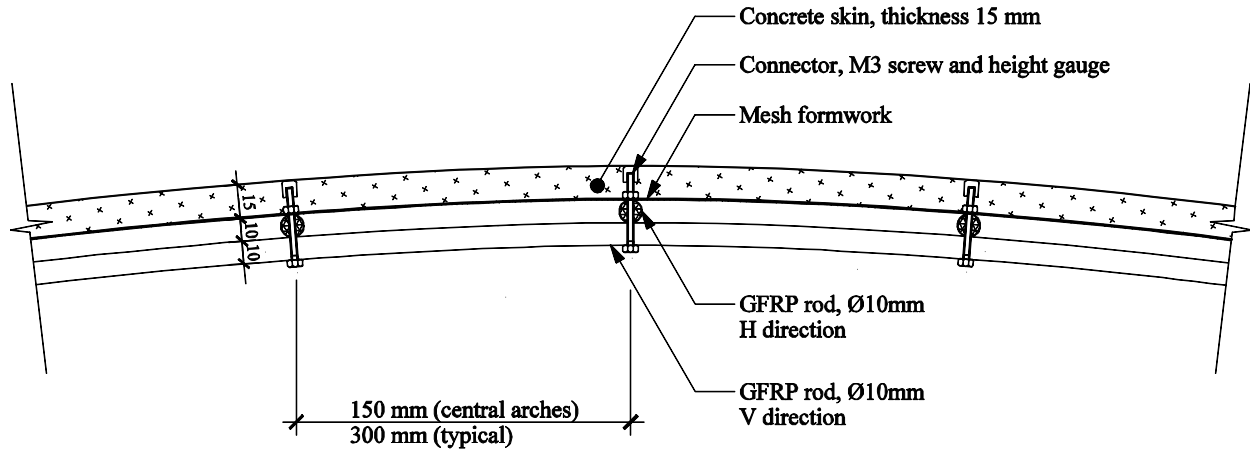
Figure 6: Section cut, typical.
