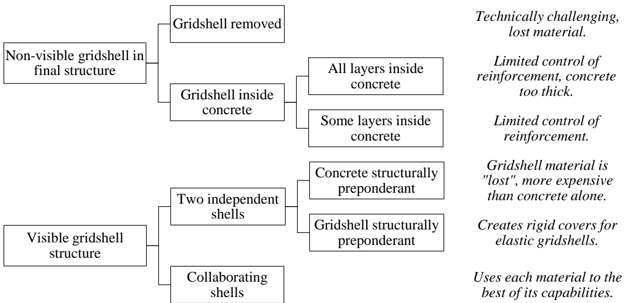
Figure 3: Taxonomy of the possible interactions between an elastic gridshell and a concrete layer.
