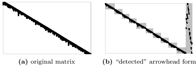
Fig. 2 constraint matrix of an instance of the temporal knapsack problem, (a) original and (b) “forced” into arrowhead form with k = 10 blocks.
