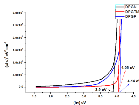
Fig. 4. Tauc's plot between (\alpha hv)^2 and (hv) .
