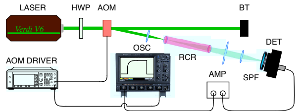
Figure 3: Experimental set-up. LASER : single longitudinal mode Nd: YVO 4 laser (Verdi V6, Coherent) delivering a cw at 532 nm; HWP, half-wave plate; AOM, acousto-optic modulator (AA Opto-Electronic, MTS110-A-VIS); BT, beam trap absorbing the non-diffracted light; RCR, ruby crystal rod; SPF, dichroic shortpass filter (Semrock: BSP-633R-25) eliminating the ruby fluorescence light at 694 nm; DET, high-speed silicon photodetector (Thorlabs DET 210, DC-350MHz); AMP, low-band (DC-200 kHz) amplifier (Hamamatsu C7319); OSC, digital oscilloscope (Lecroy Waverunner 104 MXi); AOM DRIVER, function generator driving the acousto-optic modulator and triggering the oscilloscope.
