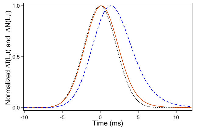
Figure 1: Normalized transmitted pulse \Delta I(L, t) (solid line) and population variation \Delta N(L, t) (dashed line). Parameters: \bar{I}(0) = 0.23 , T_1 = 1.6 ms, \alpha = 1.17 cm -1 and L = 4.25 cm, leading to \alpha L \approx 5 , \bar{I}(L) \approx 2 \times 10^{-3} , T_L \approx T_1 , \Delta\tau_g(L) \approx T_1 and \tau_{gmod}(L) \approx 0.3 ms. The normalized incident pulse \Delta I(0, t) (dotted line) of FWHM duration \tau_{in} = 5 ms is given for reference. Note the large delay of \Delta N(L, t) compared to that of \Delta I(L, t) .
