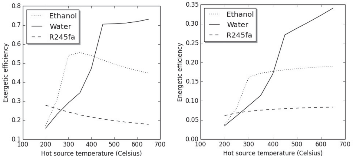
Fig. 11. Exergetic efficiency ( \eta_{II} ) of Hirm cycle without constraints. Cycle with super-heating.
