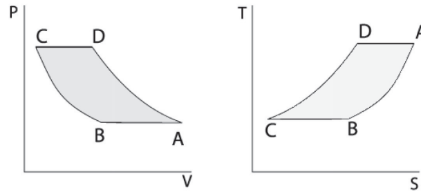
Fig. 5. Schematic diagram of Ericsson cycle
