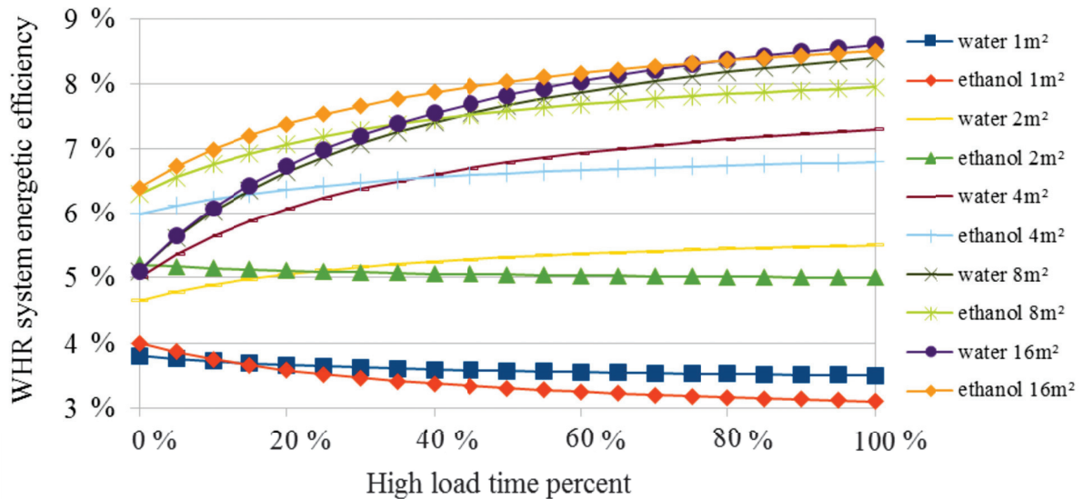
Fig. 14. Energy efficiency of waste heat recovery system as a function of the evaporator surface, fluid and high load operating time percent
