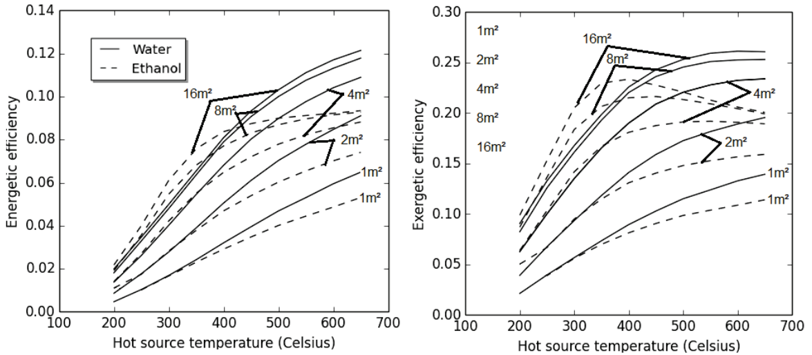
Fig. 13. Energetic and exergetic efficiency for different heat exchanger surfaces with water and ethanol for 70kW exhaust gas power.
