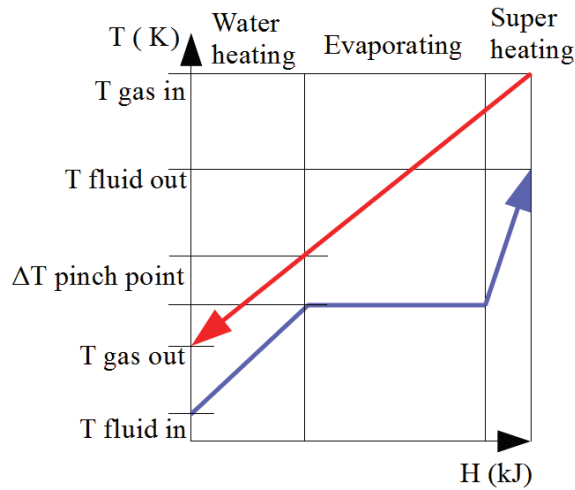
Fig. 10. Temperature evolution in the hot heat exchanger according to enthalpies exchanged
