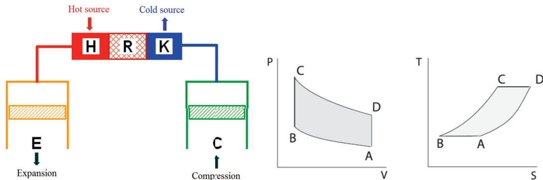
Fig. 4. Schematic diagram of Stirling engine and Stirling cycle PV and TS diagram (Juliette Bert thesis figure [6])
