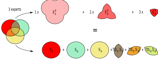
Figure 1. Illustration of the combinatorial “trick” with 3 experts
