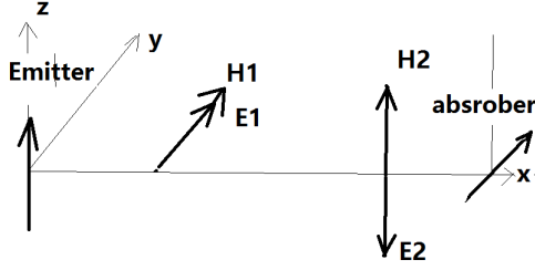
Figure 3: In this photon model, the fields \zeta_1 = [\vec{E}_1, \vec{H}_1, \vec{J}_1], \zeta_2 = [\vec{E}_2, \vec{H}_2, \vec{J}_2] do not satisfy the MEQS. However they still satisfy the mutual energy theorem.
