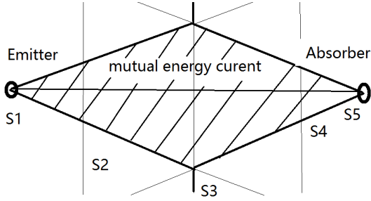
Figure 2: The mutual energy current only exists at the overlap place of the the two solutions of the MEQS. The field of the emitter is retarded wave. The wave of the absorber is advanced wave.
