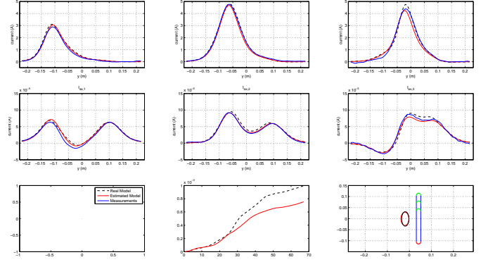
Fig. 3. Experiment using Ammari tensor with a conductive ellipsoid 33 \times 16\text{mm} with \theta_s = 0^\circ , d = 70\text{mm} . For all plots, experimental measurements are in blue, model measurements with the real object are in dotted black, and model measurements with the estimated object are in red. 1) I_{lat,1} 2) I_{lat,2} , 3) I_{lat,3} 4) \delta I_{ax,1} 5) \delta I_{ax,2} , 6) \delta I_{ax,3} , 7) Legend 8) Scores 9) Result.
