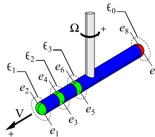
Fig. 1. Our robot equipped with 4 pairs of electrodes.
